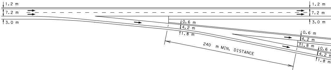
MINIMUM DISTANCE BETWEEN RAMP INTERSECTIONS
