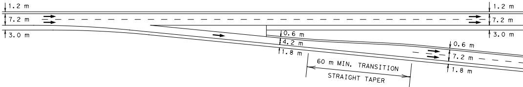
ONE LANE EXIT TRANSITION TO TWO LANE CONNECTING ROADWAY
