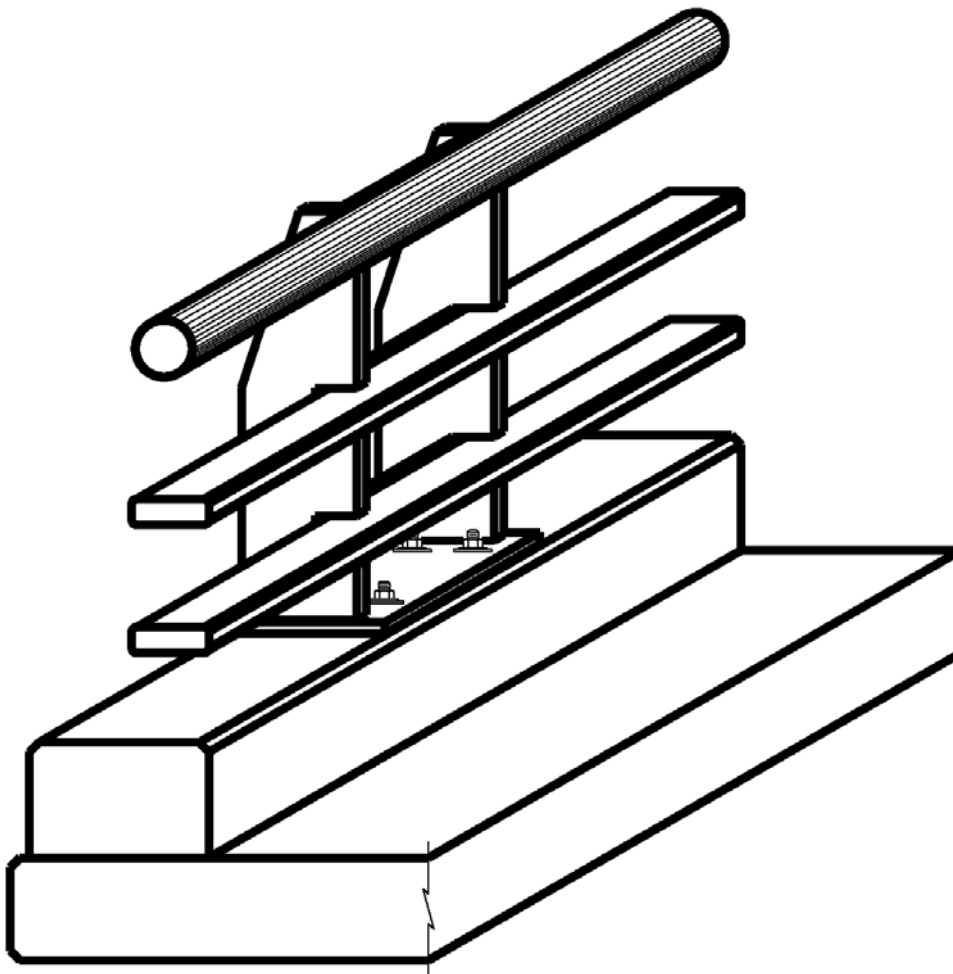
Figure A-6. Type T2P Railing
