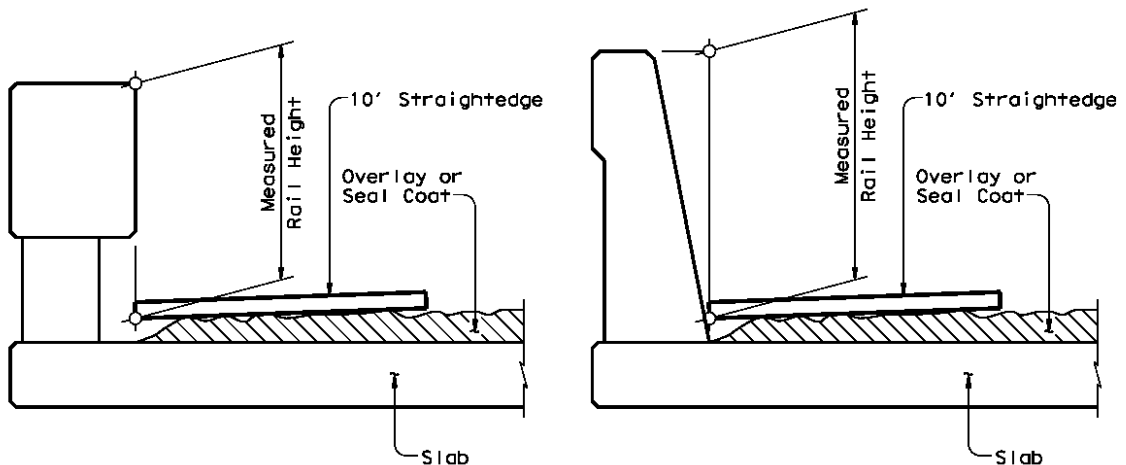
Figure 4-2. Measuring bridge railing height with overlay or seal coat
