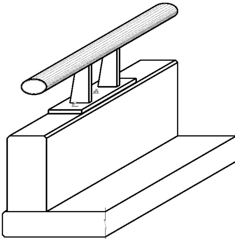
Figure A-8. Type T402 Railing
