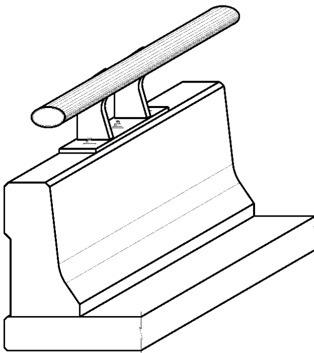
Figure A-9. Type T80HT Railing
