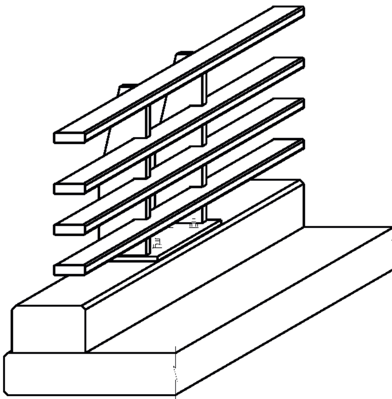
Figure A-11. Type C1W Railing
