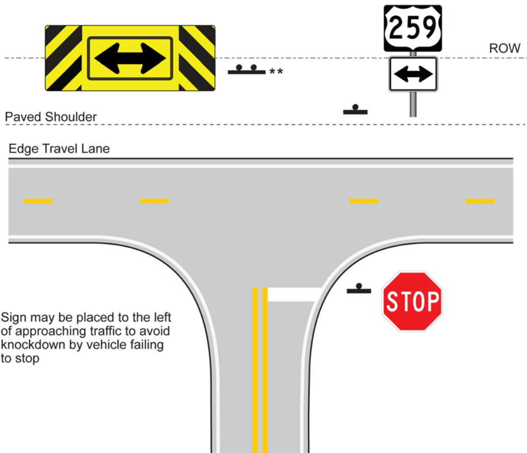
Figure 4-14. Placement of Large Arrow Panel
