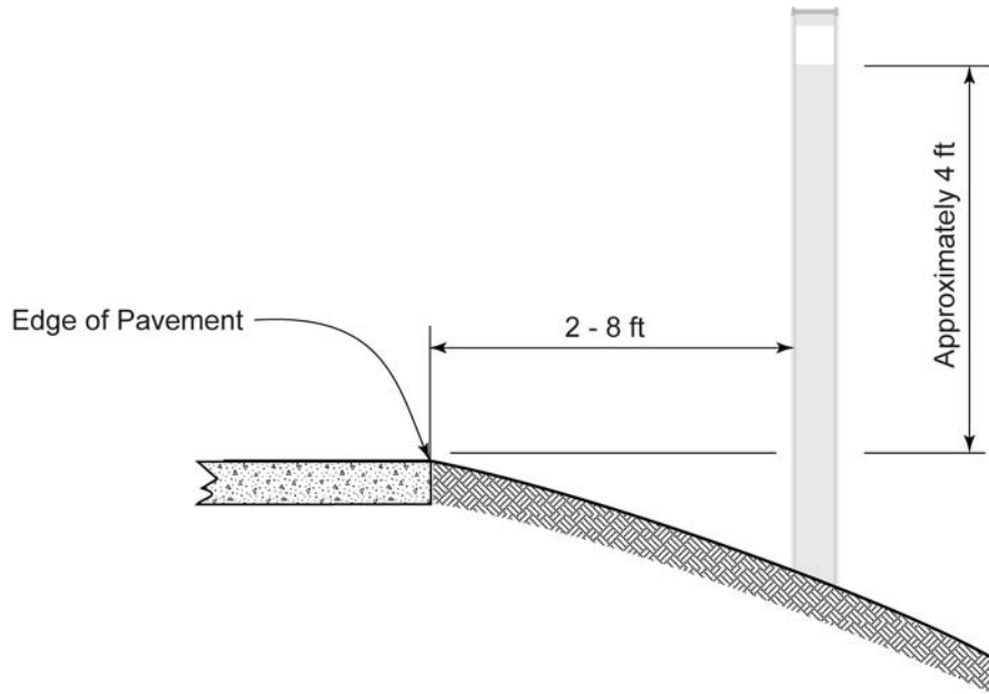
Figure 8-9. Typical Delineator Installation
