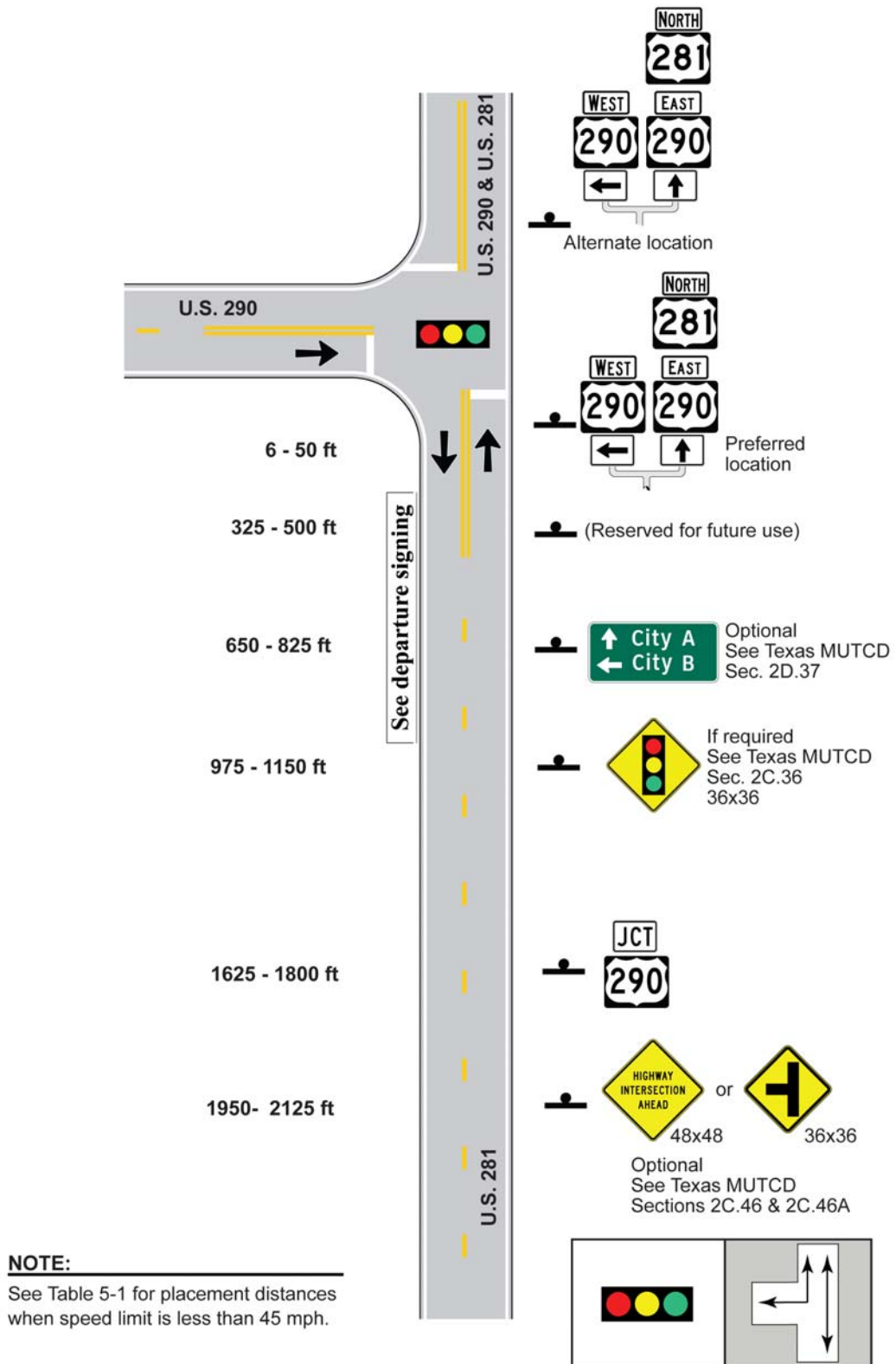
Figure 5-14. 3-Leg Side, 1 Approach Lane, Signal Control, Approach Route Goes Through
