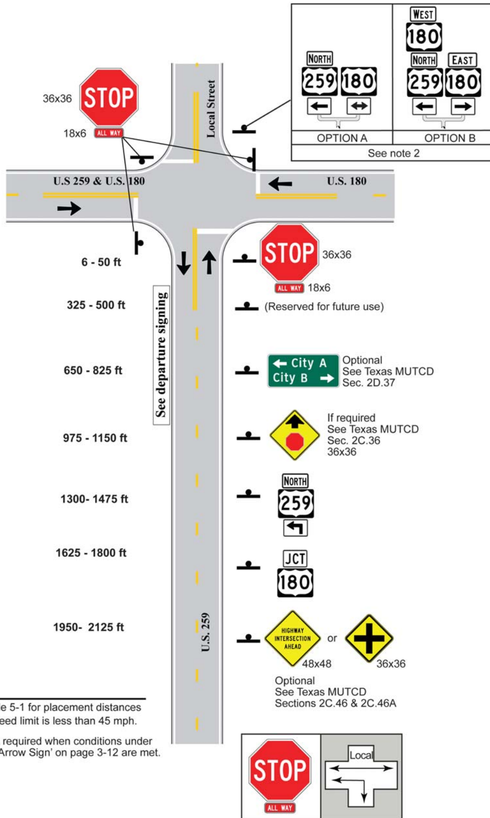
Figure 5-26. 4-Leg with Local Street, 1 Approach Lane, Stop Control, Approach Route Goes Left
