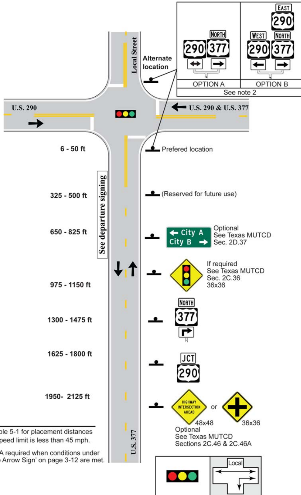
Figure 5-28. 4-Leg with Local Street, 1 Approach Lane, Signal Control, Approach Route Goes Right
