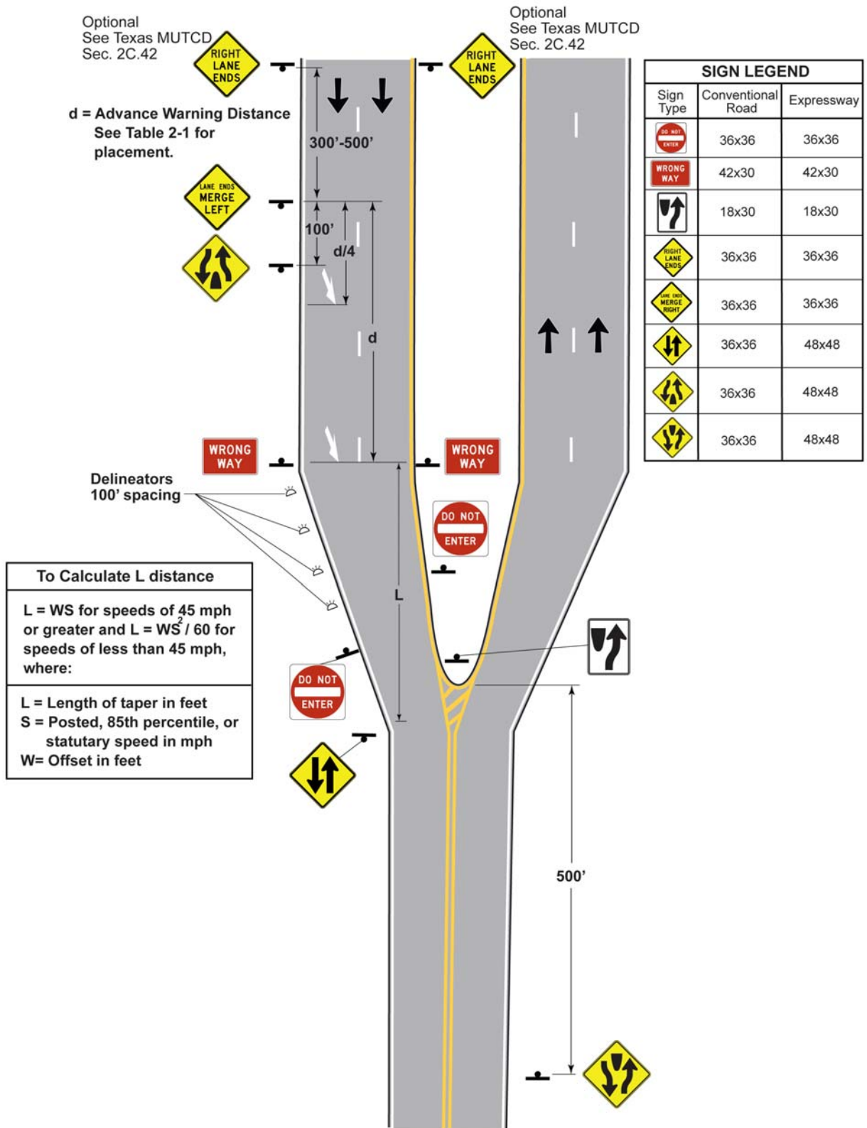
Figure 7-23. Transition to 4-Lane Divided Highway
