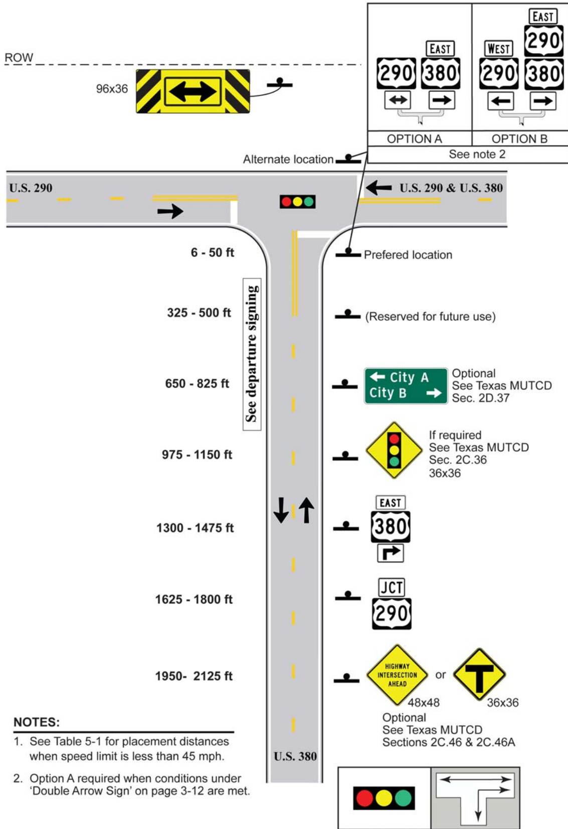
Figure 5-7. 3-Leg T, 1 Approach Lane, Signal Control, Approach Route Goes Right
