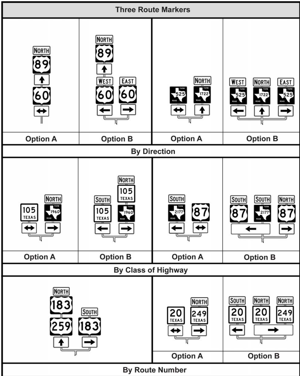
Figure 3-21. Route Sign Assembly for Intersection with Three Route Signs
