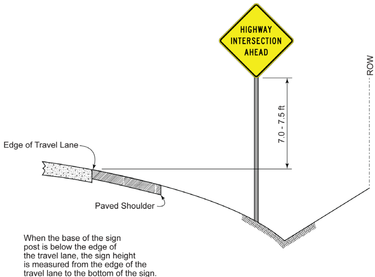
Figure 4-15. Sign Height on Front Slope
