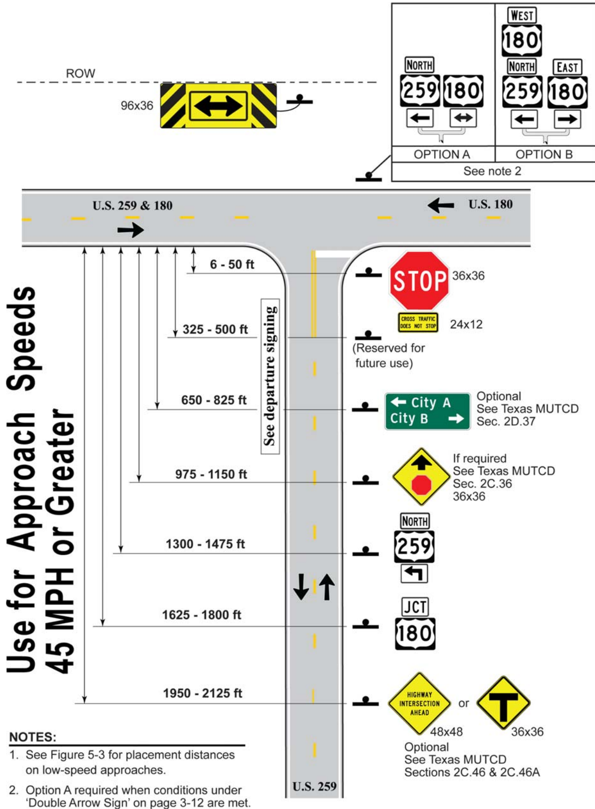
Figure 5-2. Convention for Sign Placement Distances on High-Speed Approach
