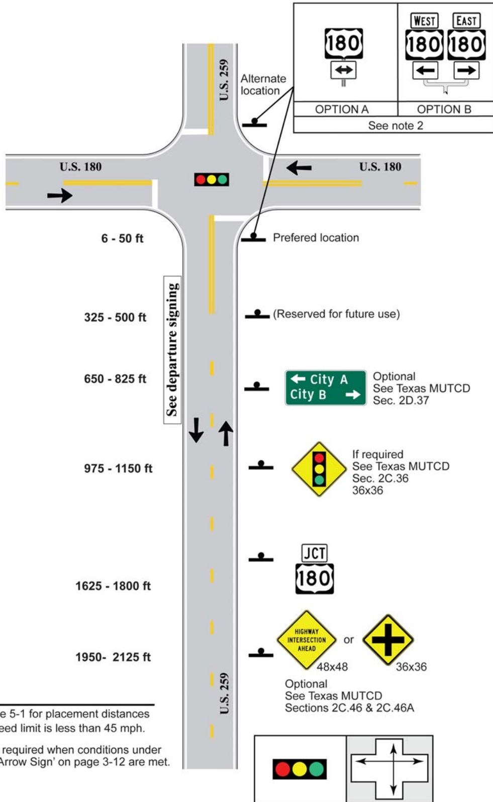
Figure 5-20. 4-Leg, 1 Approach Lane, Signal Control, Approach Route Goes Through
