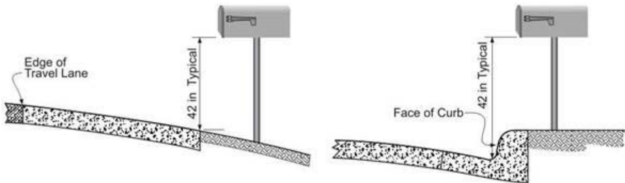
Figure 9-7. Height of Mailbox
