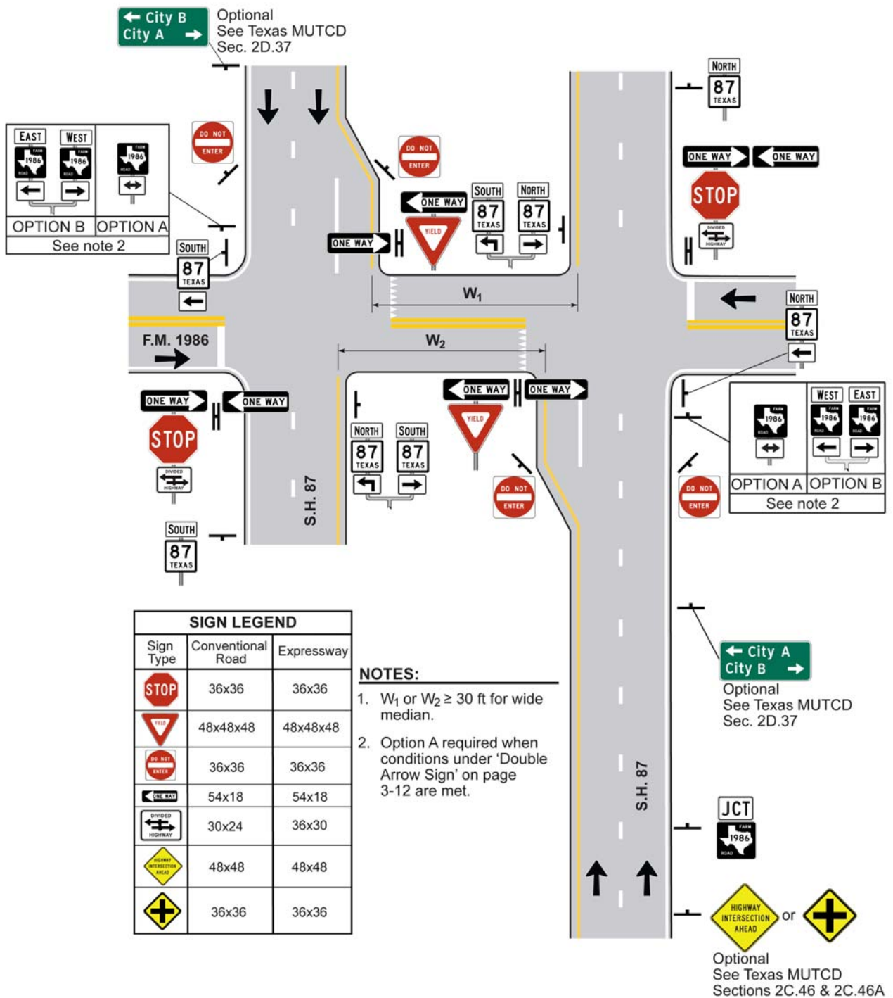
Figure 7-4. Signing for Wide Median Divided Highway Intersection with Left Turn Bays and Two External Roads
