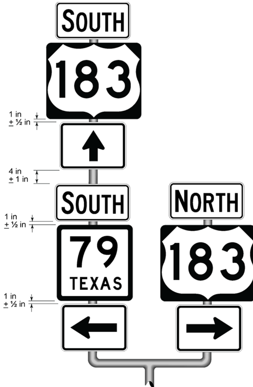
Figure 3-23. Layout Dimensions for Assemblies
