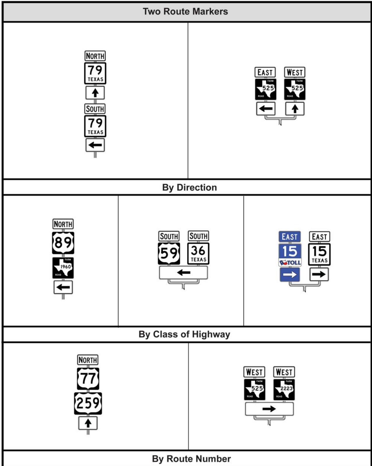
Figure 3-20. Route Sign Assembly for Intersection with Two Route Signs
