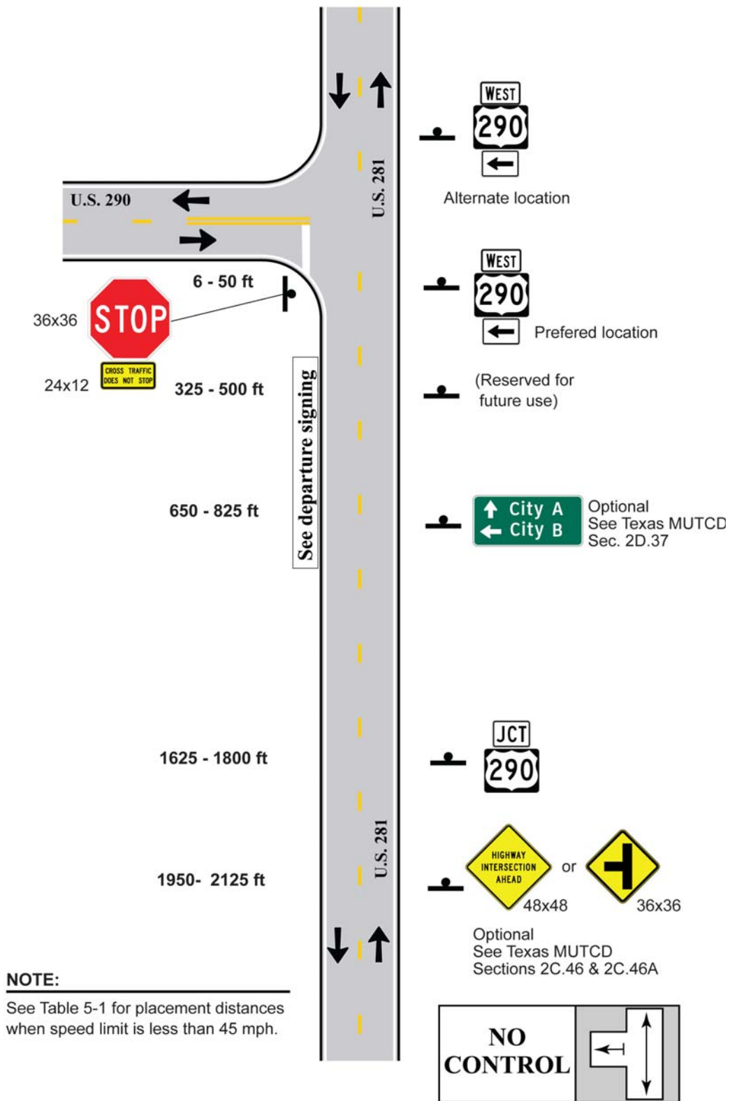
Figure 5-10. 3-Leg Side, 1 Approach Lane, No Control, Approach Route Goes Through
