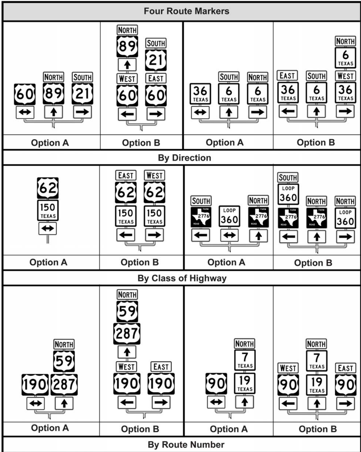
Figure 3-22. Route Sign Assembly for Intersection with Four Route Signs
