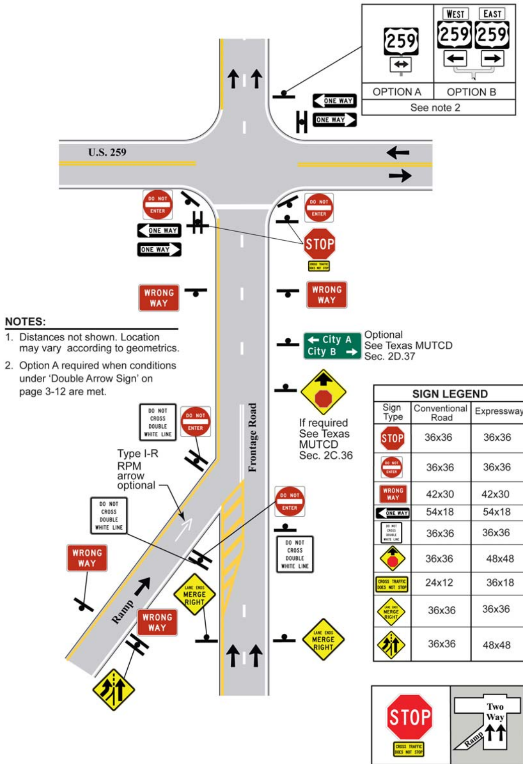
Figure 7-20. One-Way Frontage Road with Exit Ramp, Two-Lane Approach, Stop Control
