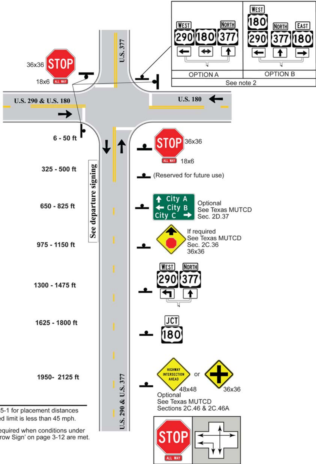
Figure 5-19. 4-Leg, 1 Approach Lane, Stop Control, Approach Route Goes Through and Left
