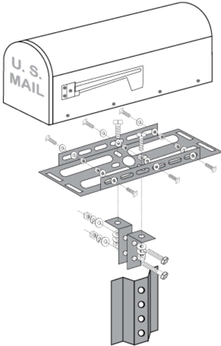
Figure 9-12. Attaching the Bracket to a Single Support
