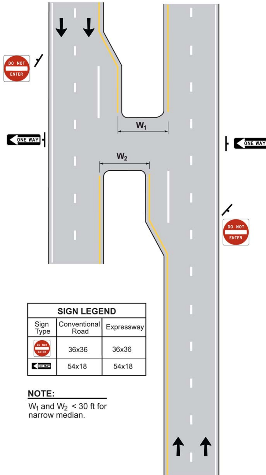
Figure 7-12. Signing for Narrow Median Crossover with Left Turn Bays
