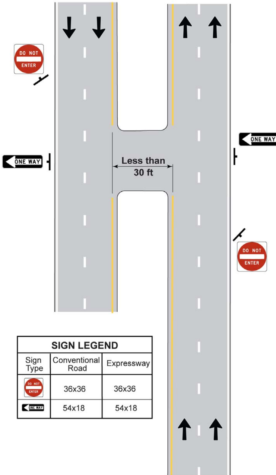
Figure 7-13. Signing for Narrow Median Crossover without Left Turn Bays
