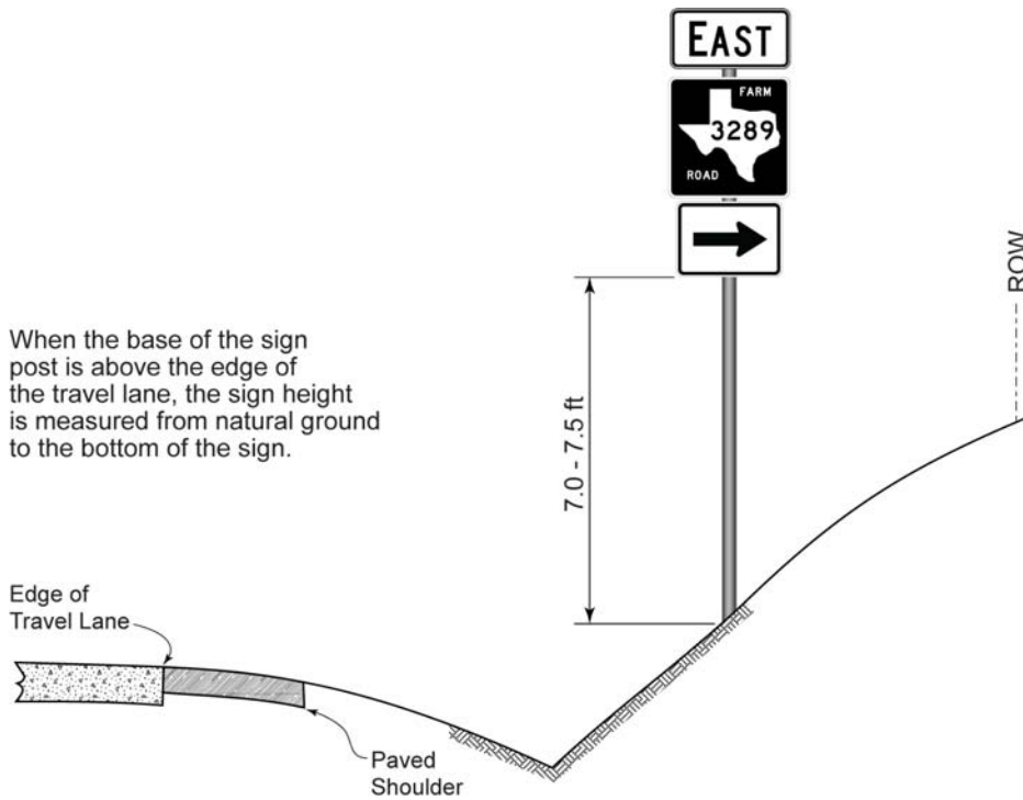
Figure 4-16. Sign Height on Back Slope
