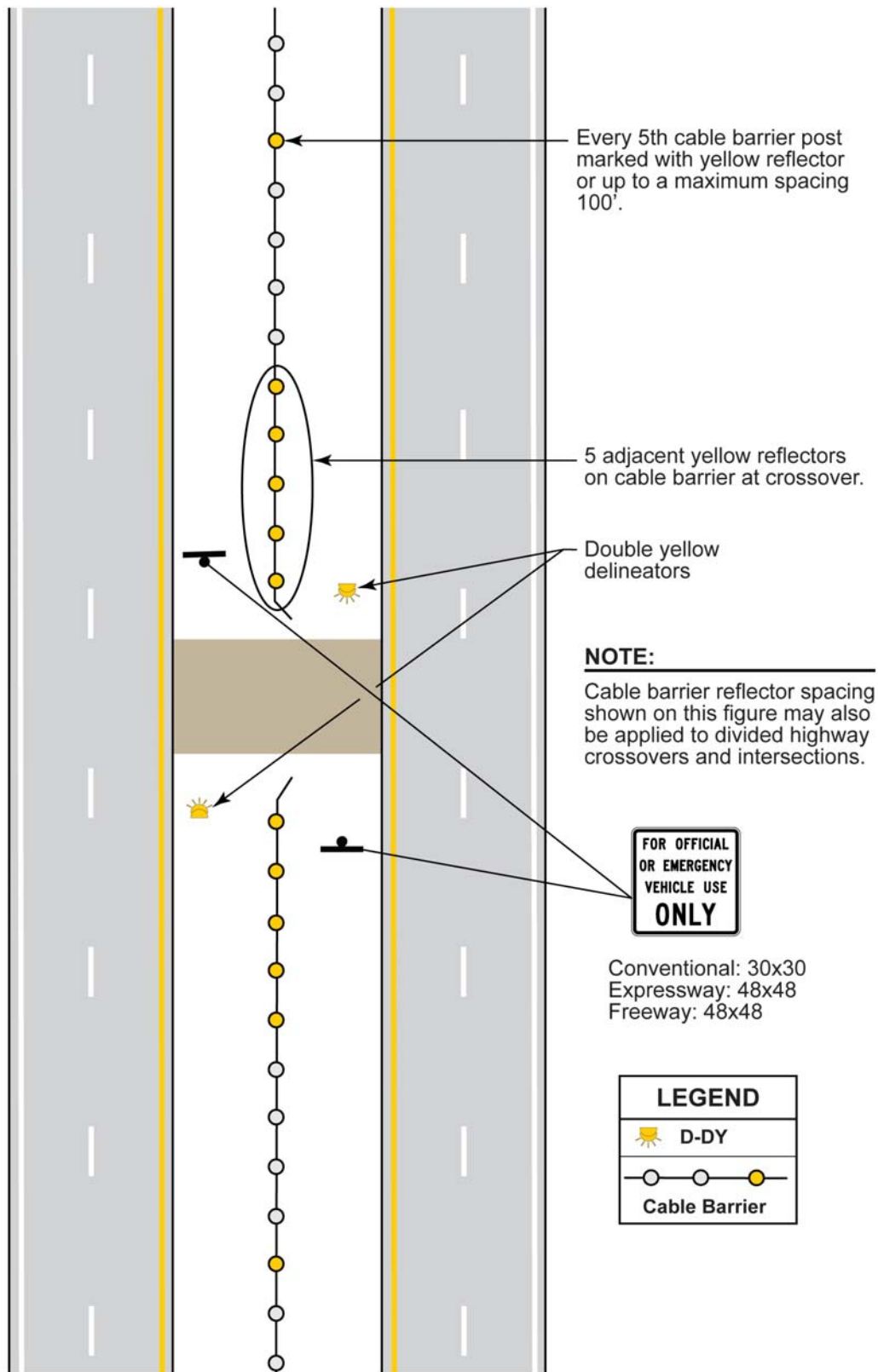
Figure 8-24. Emergency Crossover
