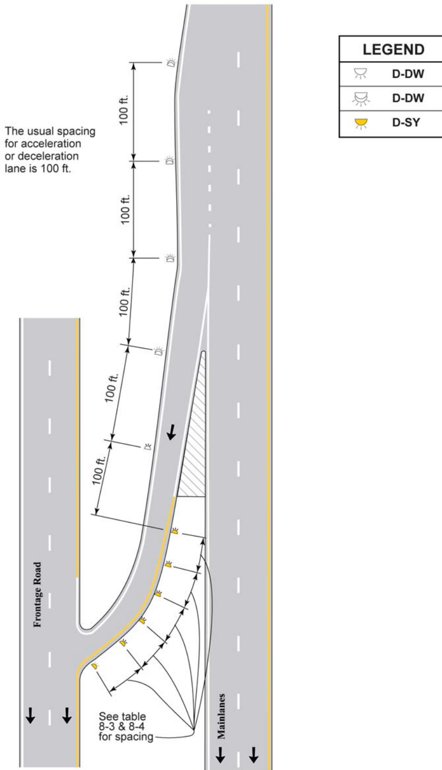
Figure 8-23. One-Way Curved Ramp Detail
