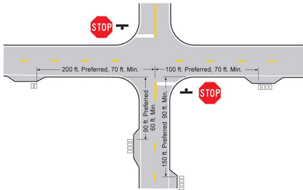
Figure 9-4. Mailbox Placement at Rural Locations: Through Highway Speed \leq 55 mph
