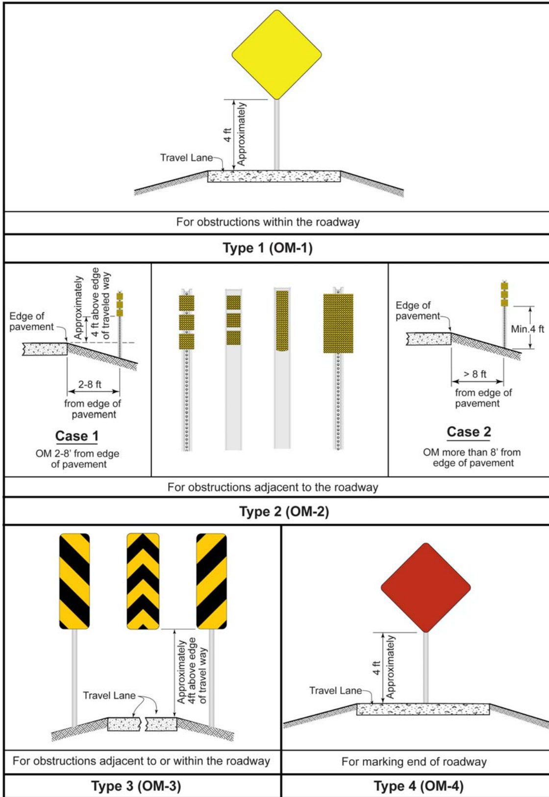
Figure 8-1. Object Markers
