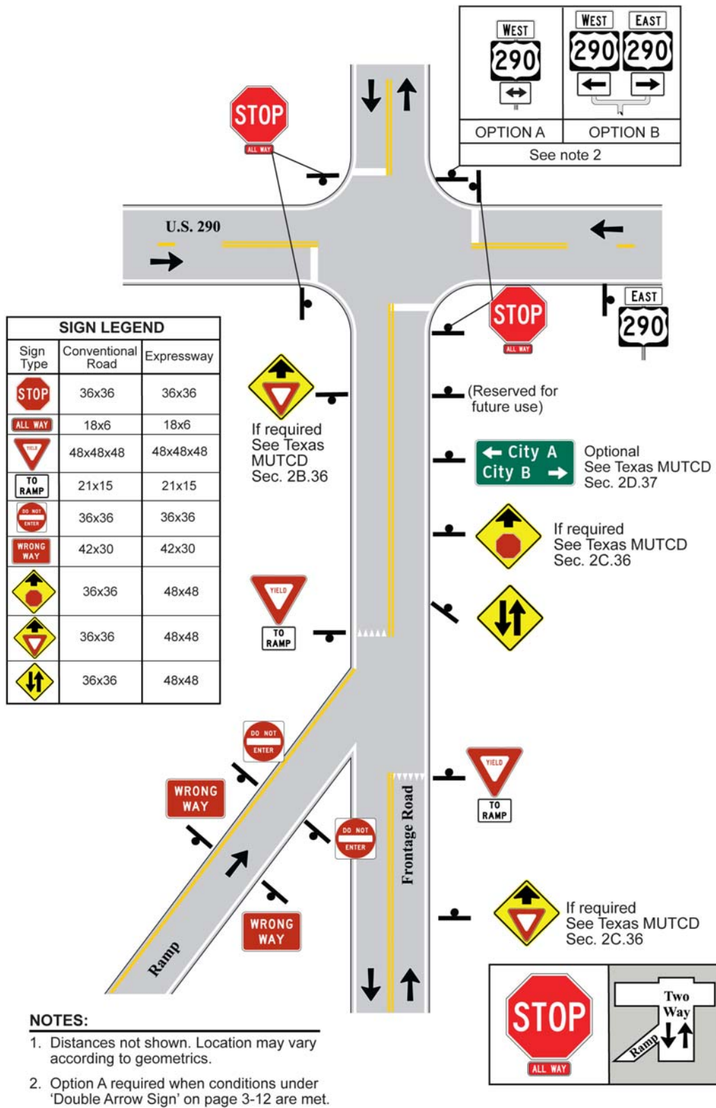
Figure 7-21. Two-Way Frontage Road with Exit Ramp, One-Lane Approach, Stop Control
