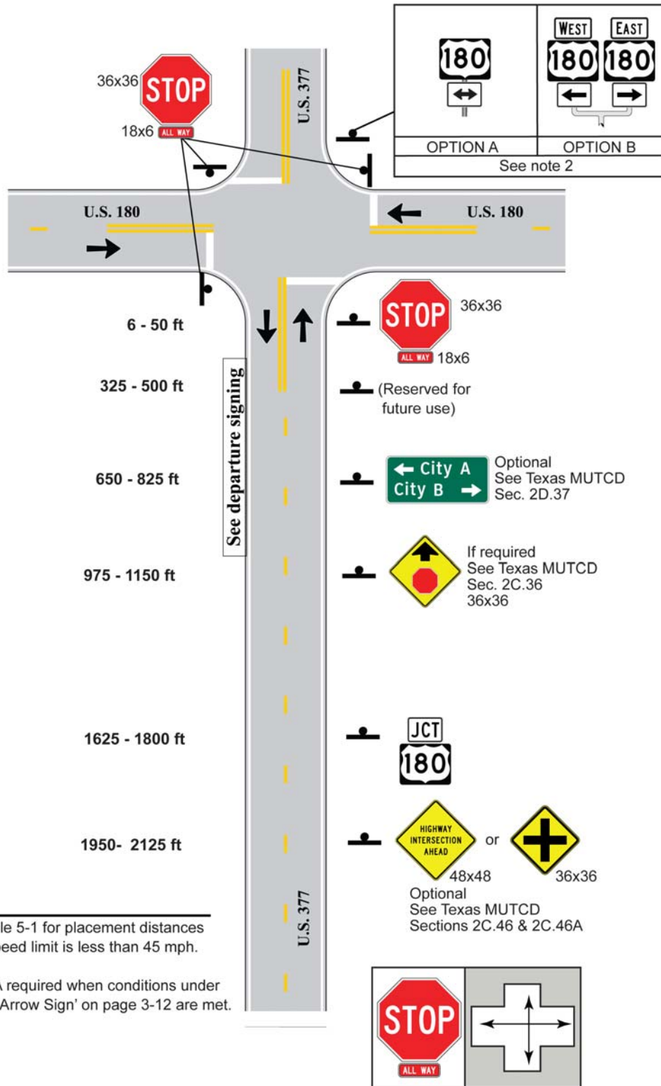
Figure 5-17. 4-Leg, 1 Approach Lane, Stop Control, Approach Route Goes Through
