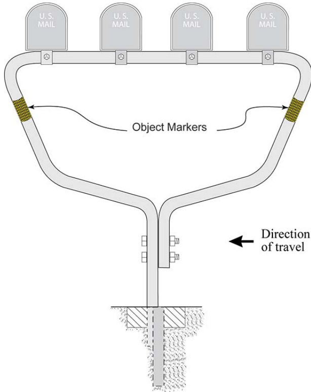
Figure 9-8. Coat Hanger Multiple Support
