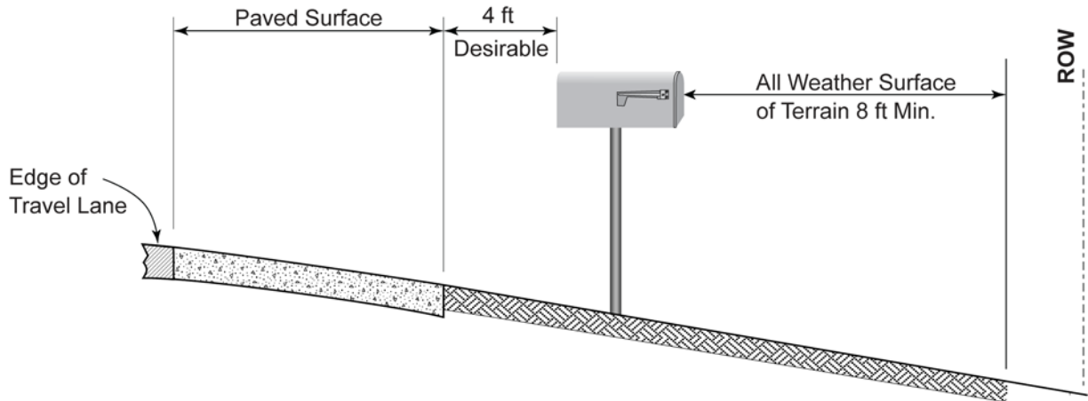
Figure 9-6. Lateral Placement for Delivery to the Back Side
