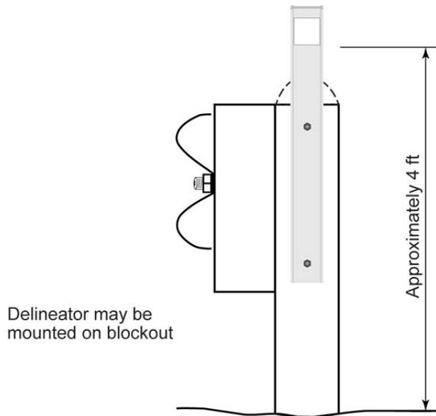
Figure 8-10. Delineator Installation on Guardrail Post
