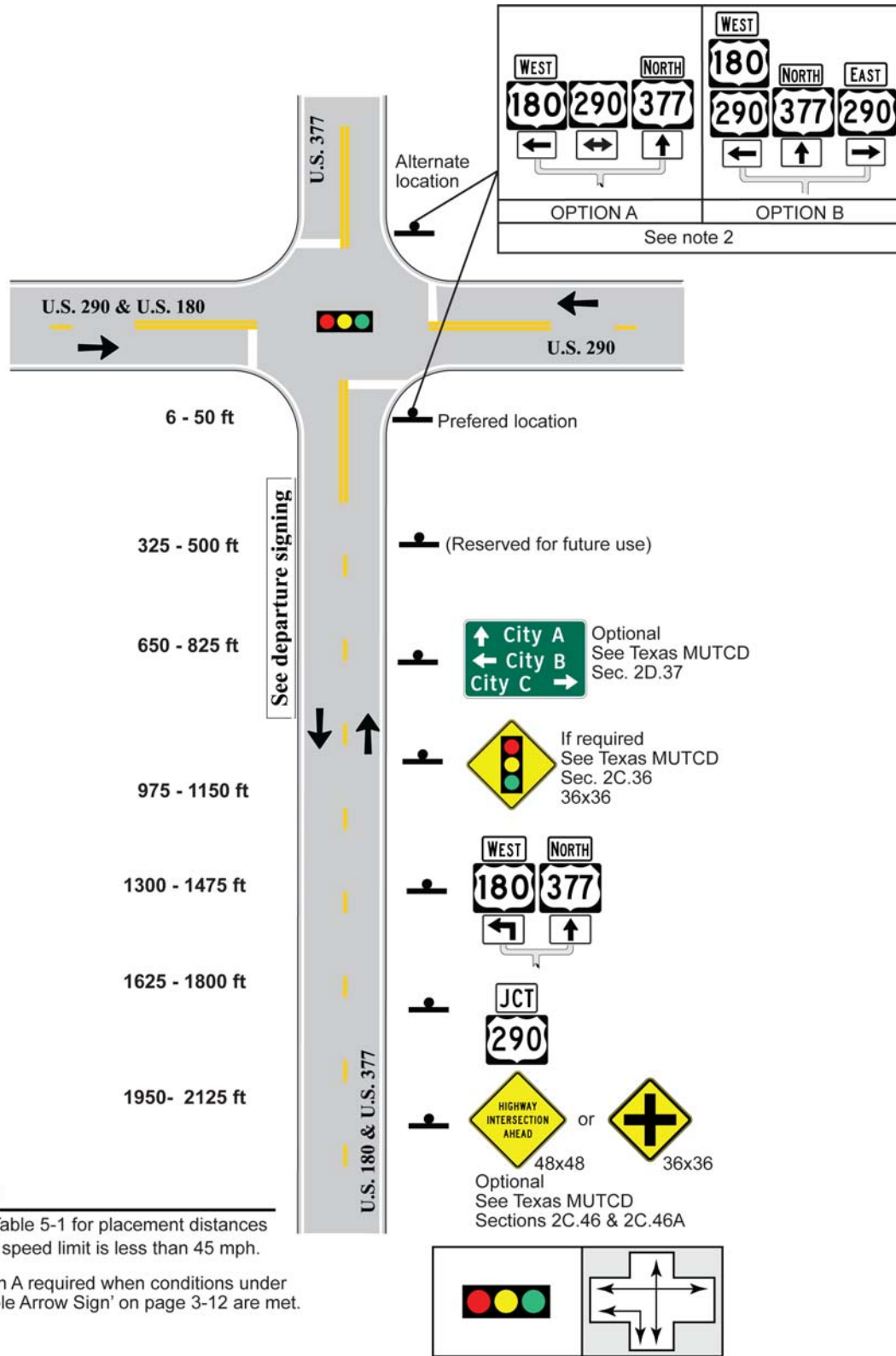
Figure 5-22. 4-Leg, 1 Approach Lane, Signal Control, Approach Route Goes Through and Left
