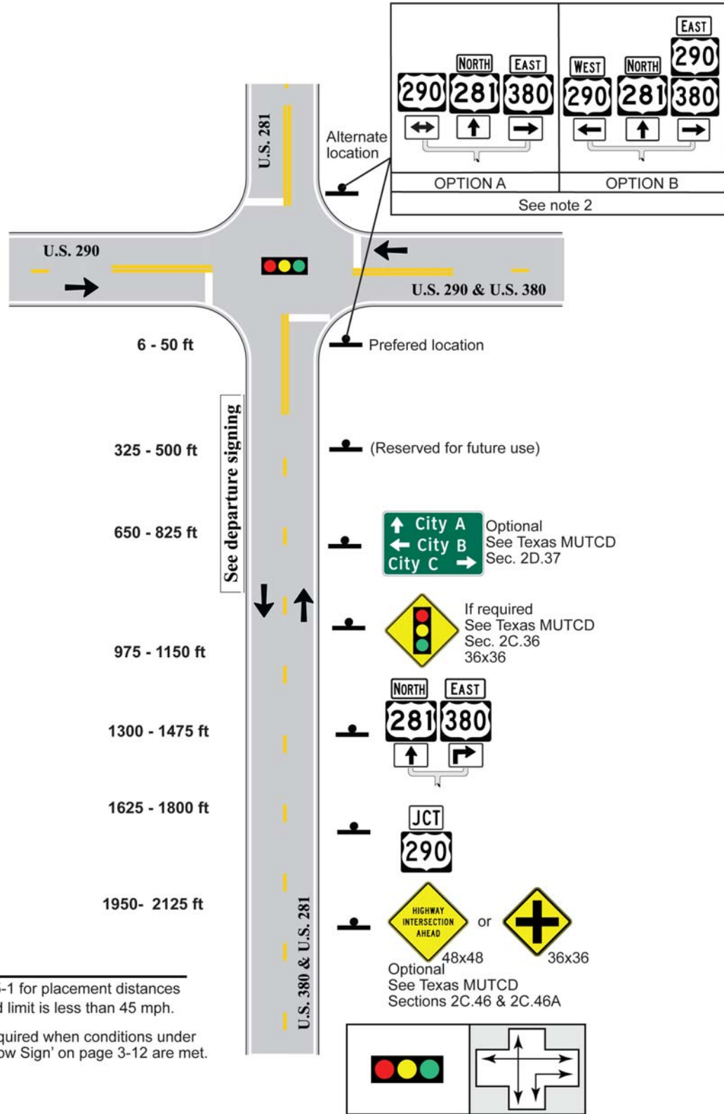
Figure 5-21. 4-Leg, 1 Approach Lane, Signal Control, Approach Route Goes Through and Right
