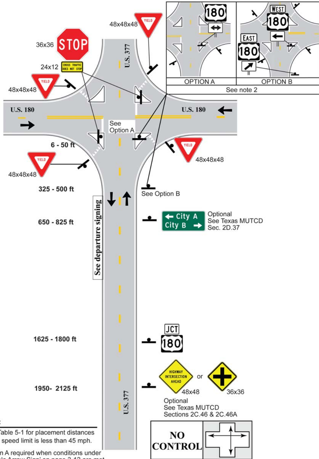
Figure 5-18. 4-Leg, 1 Approach Lane with Free Right Turn, No Control, Approach Lane Goes Through
