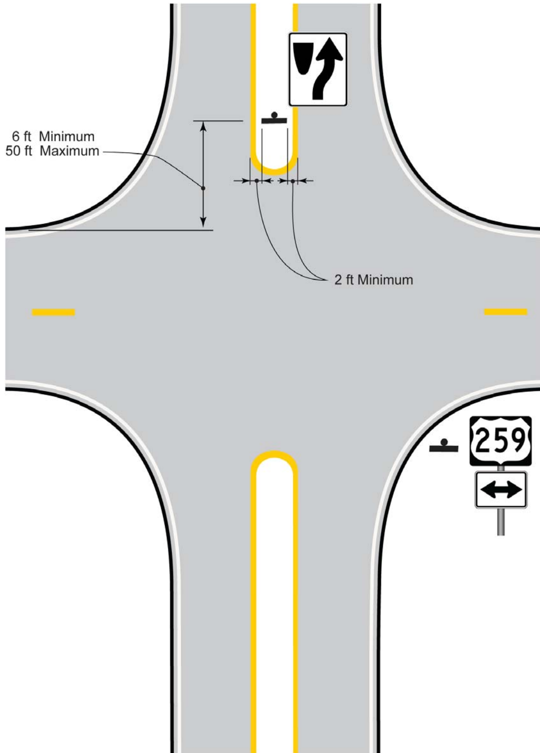
Figure 4-13. Keep Right Sign Lateral Placement on a Divisional Island
