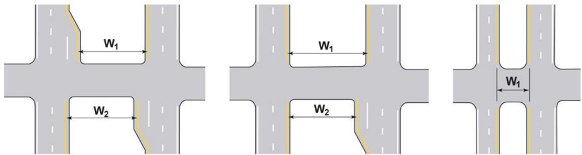
Figure 7-2. Measuring Median Width
