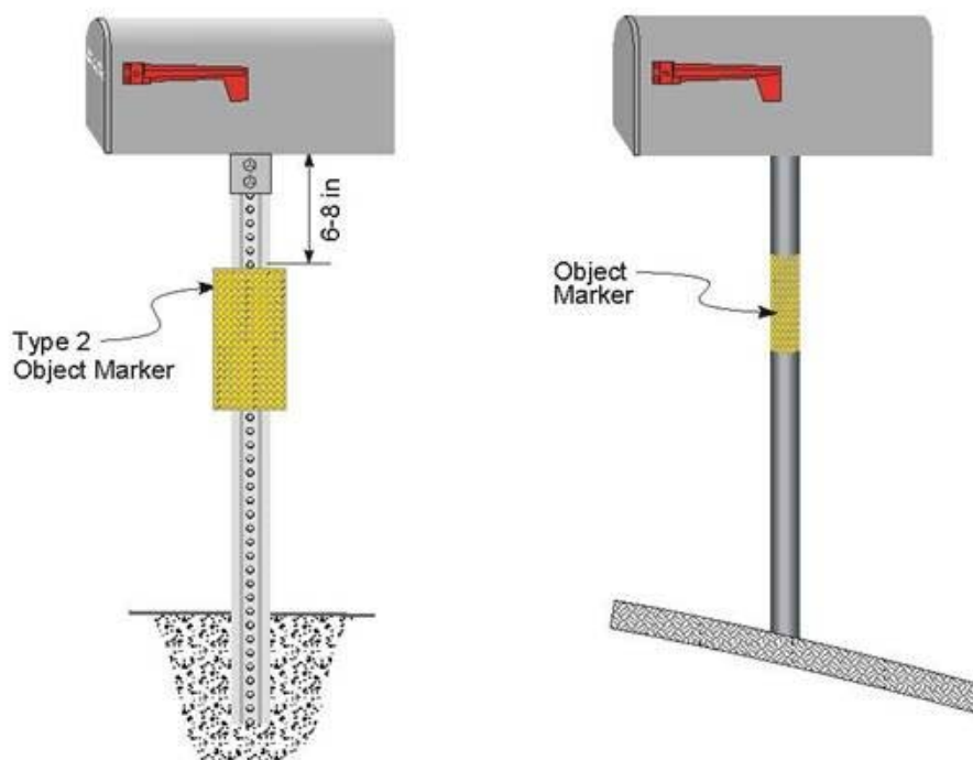
Figure 9-19. Type 2 Object Marker Installations
