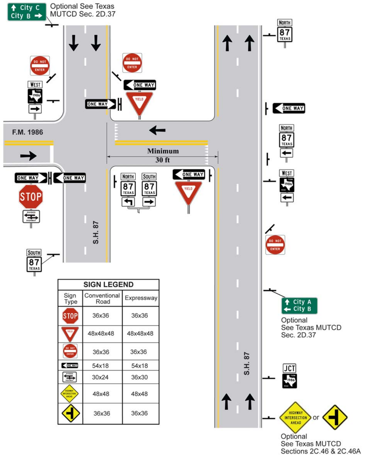
Figure 7-5. Signing for Wide Median Divided Highway Intersection without Turn Bays and One External Road
