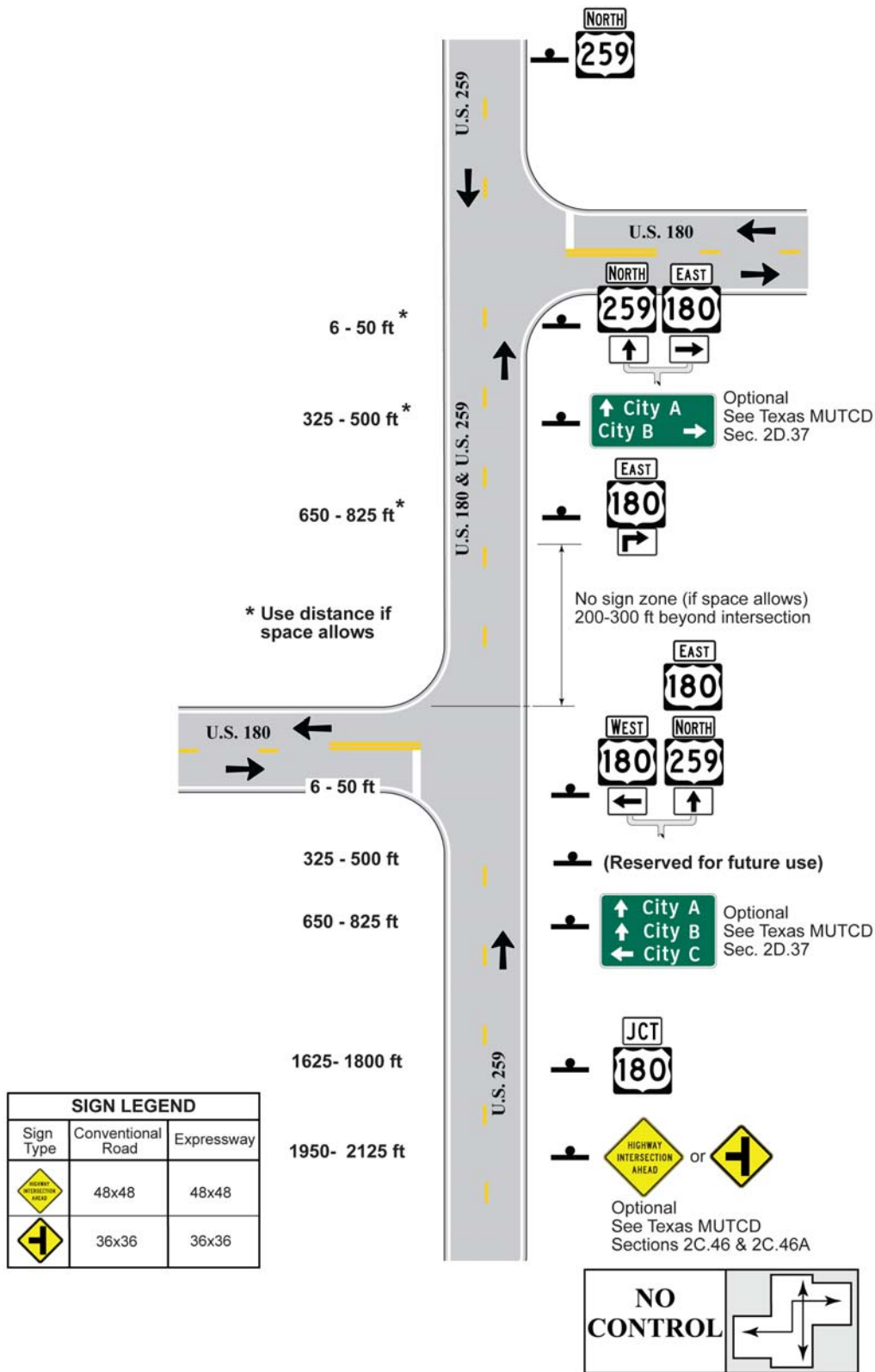
Figure 7-14. Signing for Offset Side T Intersections with Overlapping Routes
