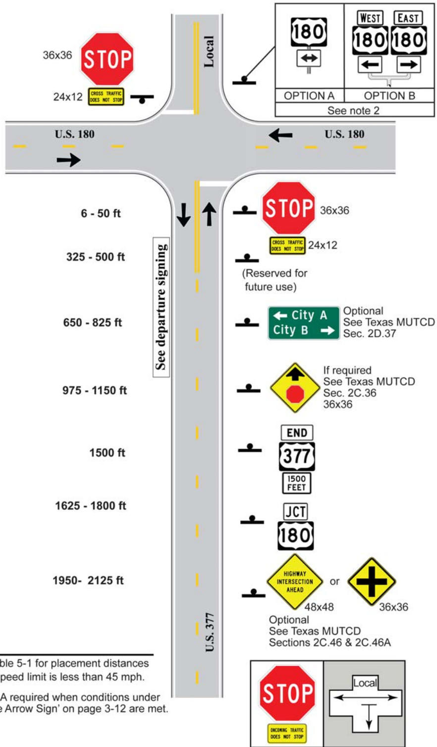
Figure 5-25. 4-Leg with Local Street, 1 Approach Lane, Stop Control, Approach Route Ends
