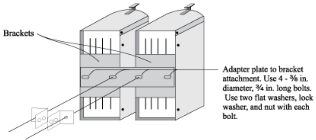
Figure 9-13. Use of the Adapter Plate for a Double Mailbox Installation
