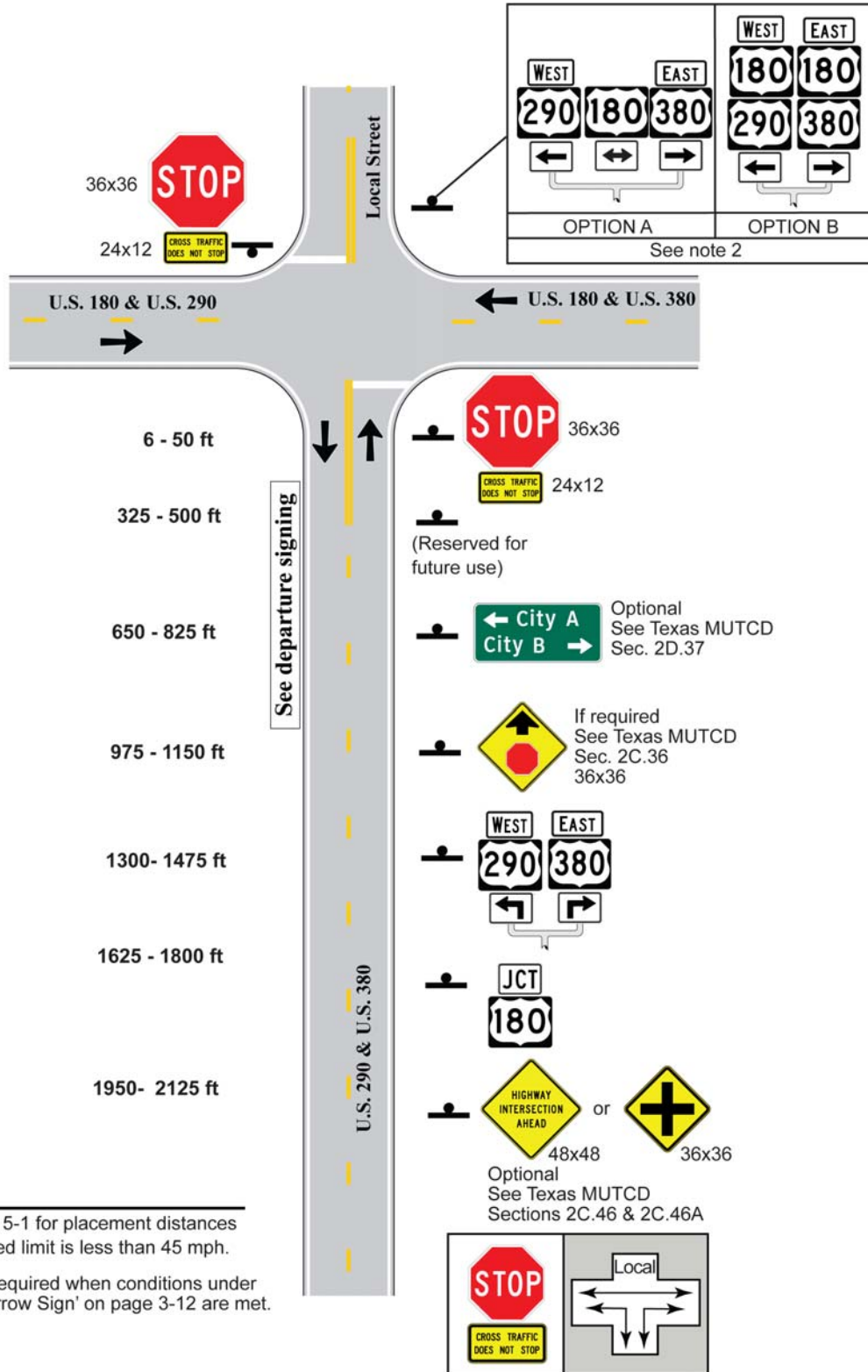
Figure 5-27. 4-Leg with Local Street, 1 Approach Lane, Stop Control, Approach Route Goes Left and Right
