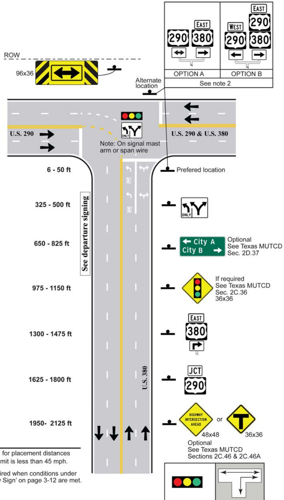
Figure 5-9. 3-Leg T, 2 Approach Lanes with Dual Left, Signal Control, Approach Route Goes Right
