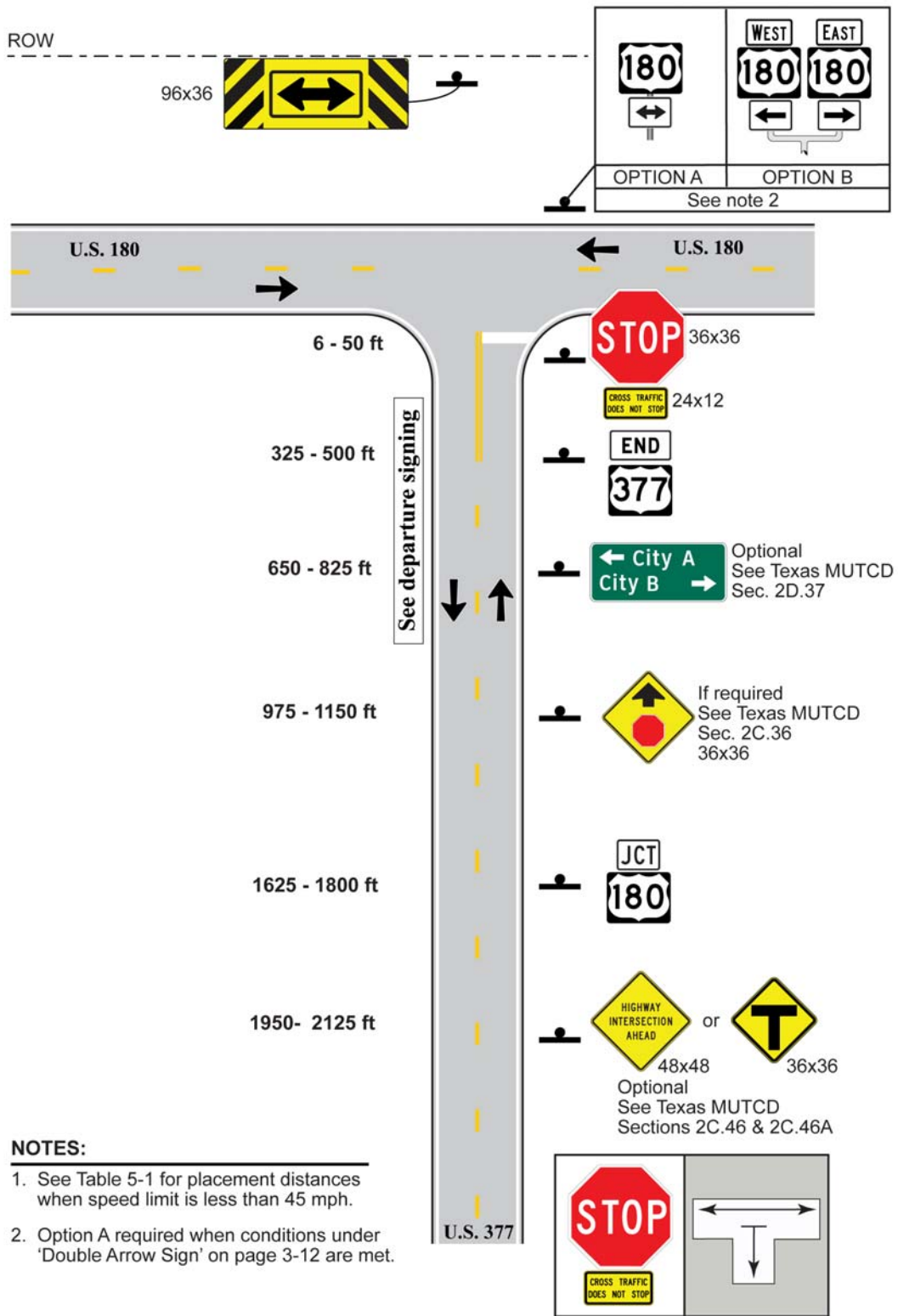
Figure 5-6. 3-Leg T, 1 Approach Lane, Stop Control, Approach Route Ends
