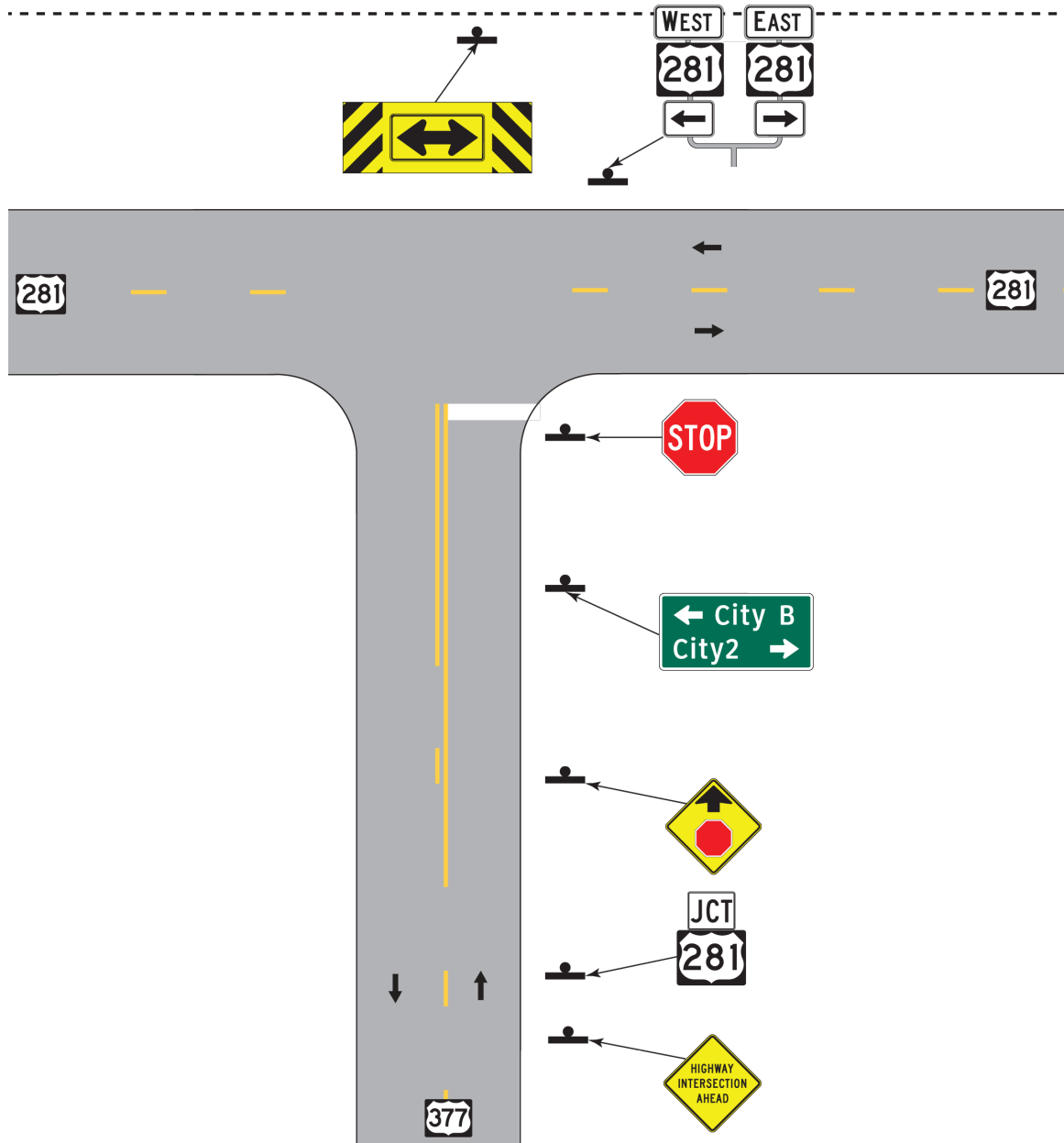
Figure 6-1. T-intersection treatments. If the large arrow sign is used, it should be as close to the ROW line as practical.
