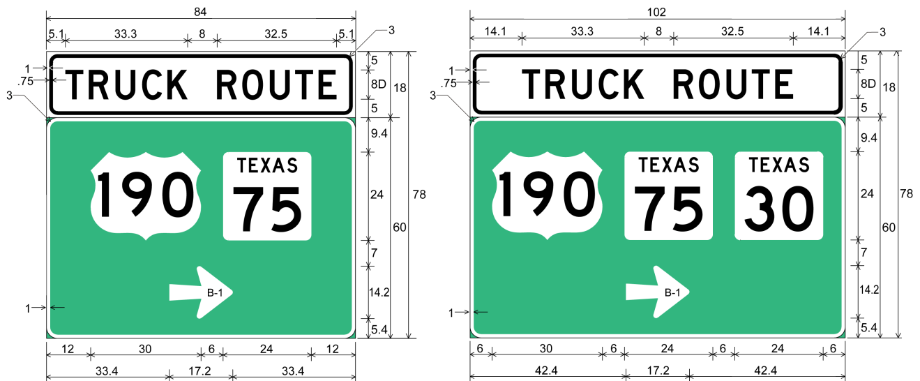
Figure 5-4. Large Advanced Truck Route Sign Assembly sign details
