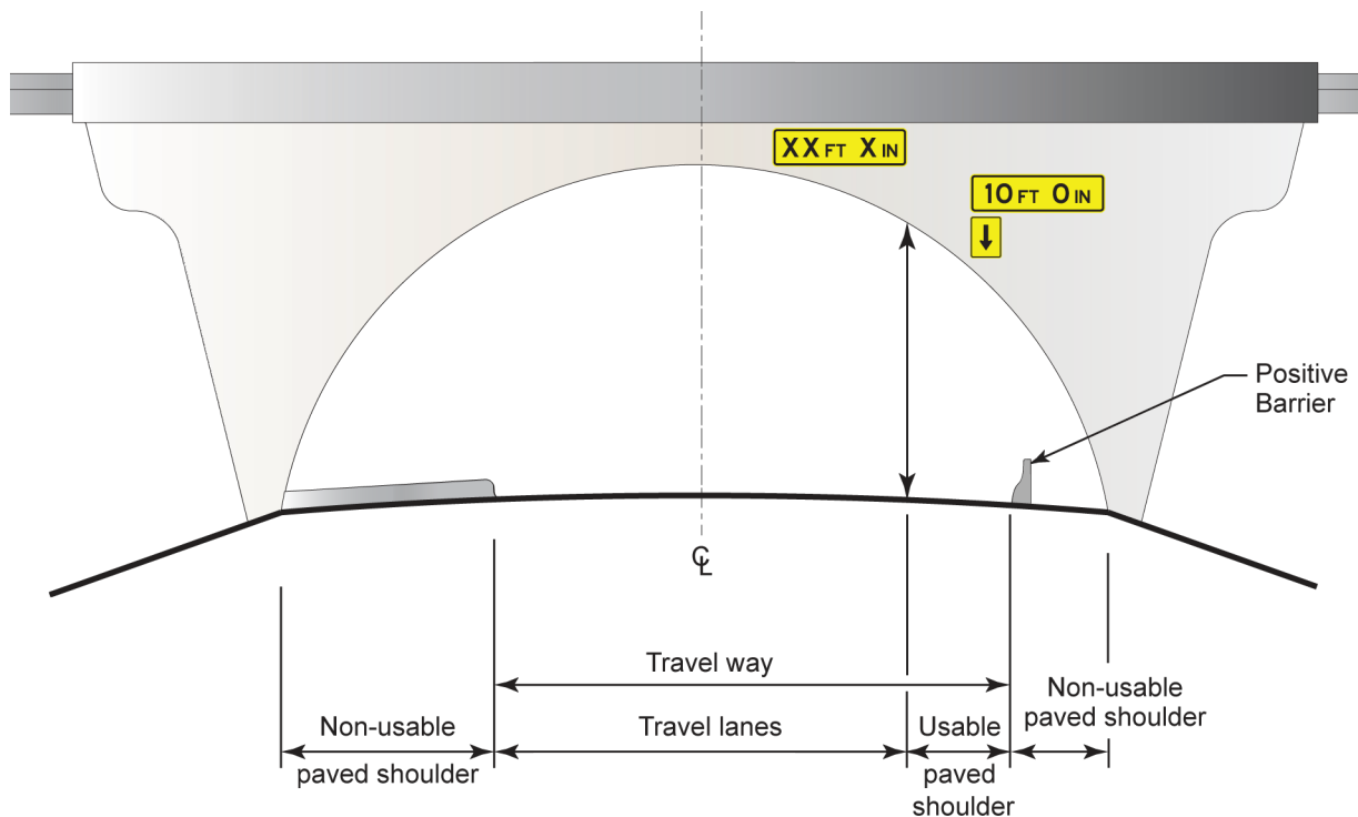
Figure 6-2. Measuring minimum vertical clearance
