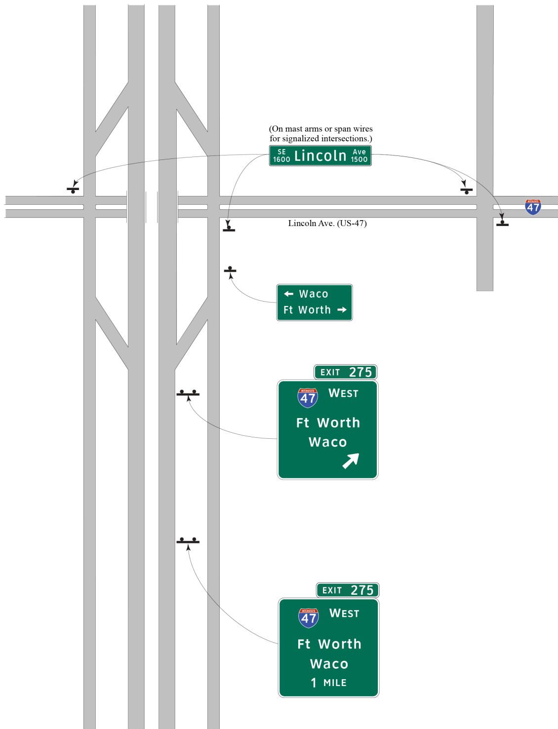
Figure 7-8. Typical signing on an expressway or freeway for an intersected highway route that is a named city street (For information on oversized street named signs at intersections, see Section 3 of this chapter.)
