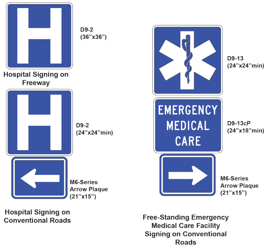
Figure 7-6. Signing for Emergency Medical Services
