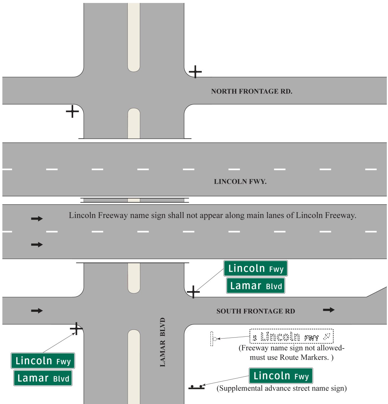
Figure 7-10. Street signs on city street for named freeway route
