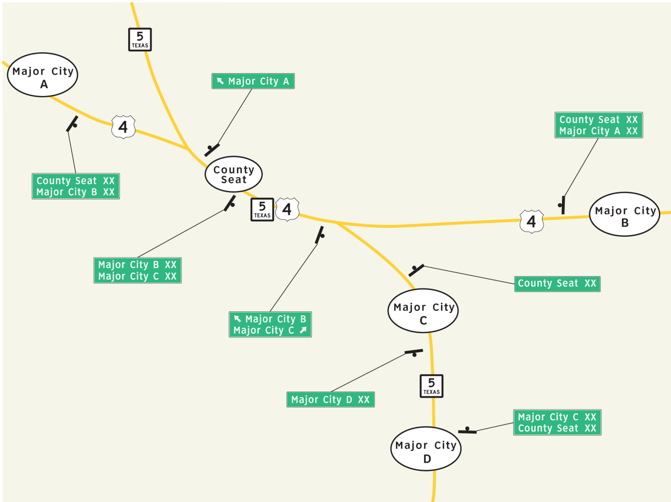
Figure 7-4. Example of supplemental destination distance signing
