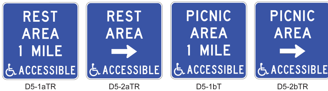
Figure 7-19. Advance and directional rest area signs (D5 series) for conventional highways showing ADA accessible message
