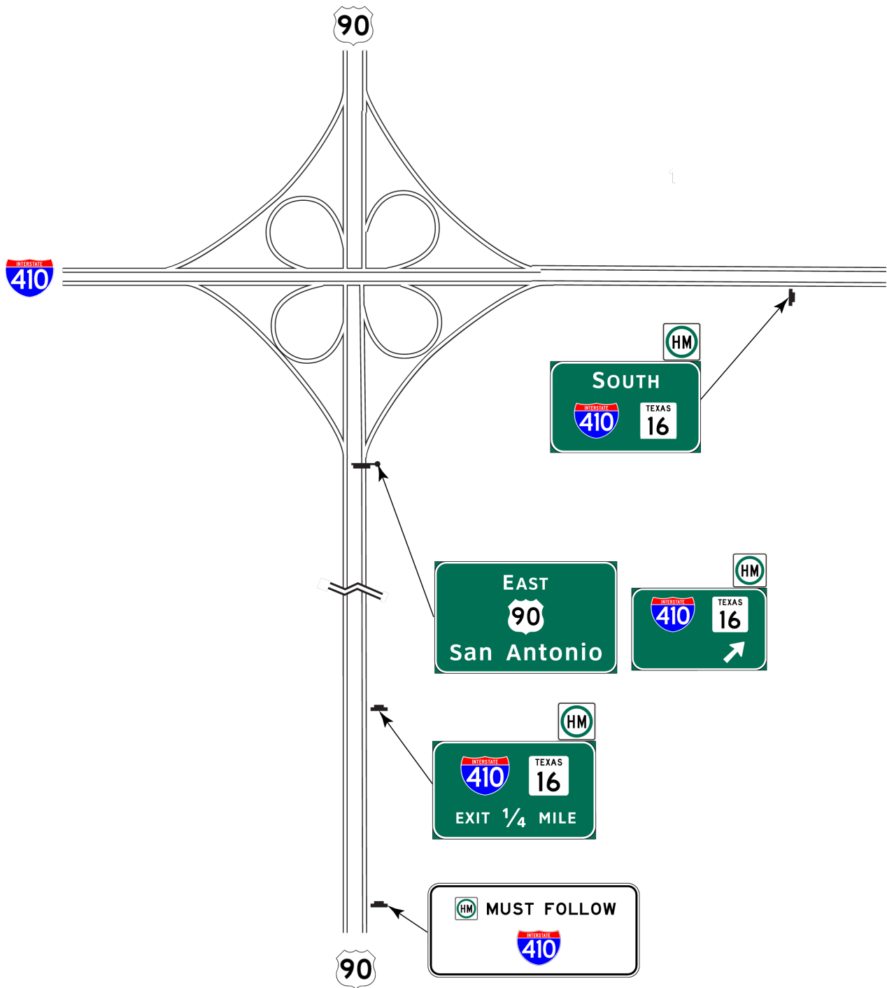
Figure 5-6. Typical signing for a designated through NRHM route on an expressway or freeway
