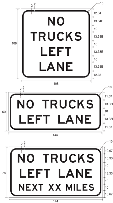
Figure 5-9. Restricted truck lane sign details
