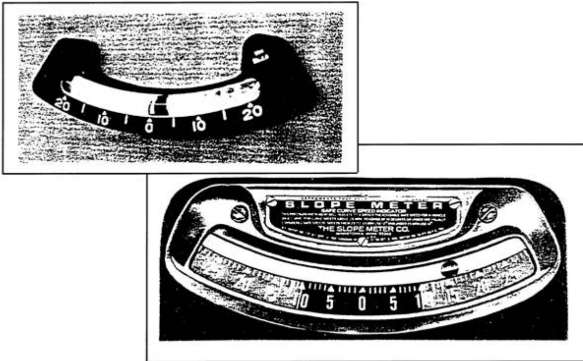
Figure 5-7. Two types of ball-bank indicators.
