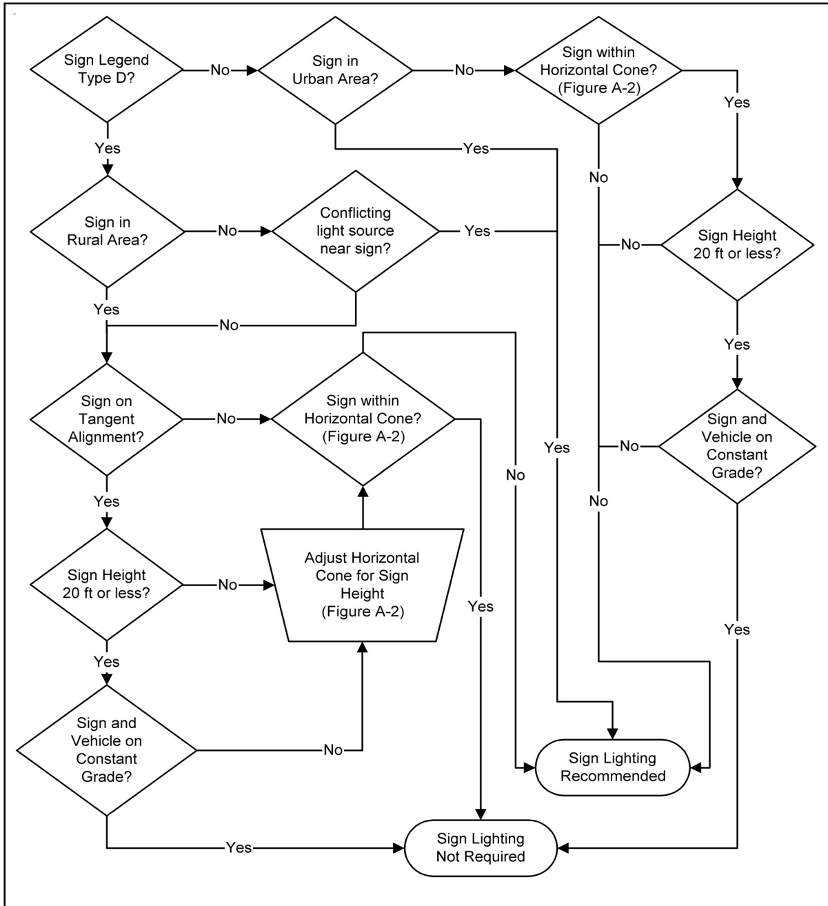
Figure A-2. Sign lighting flow chart.
