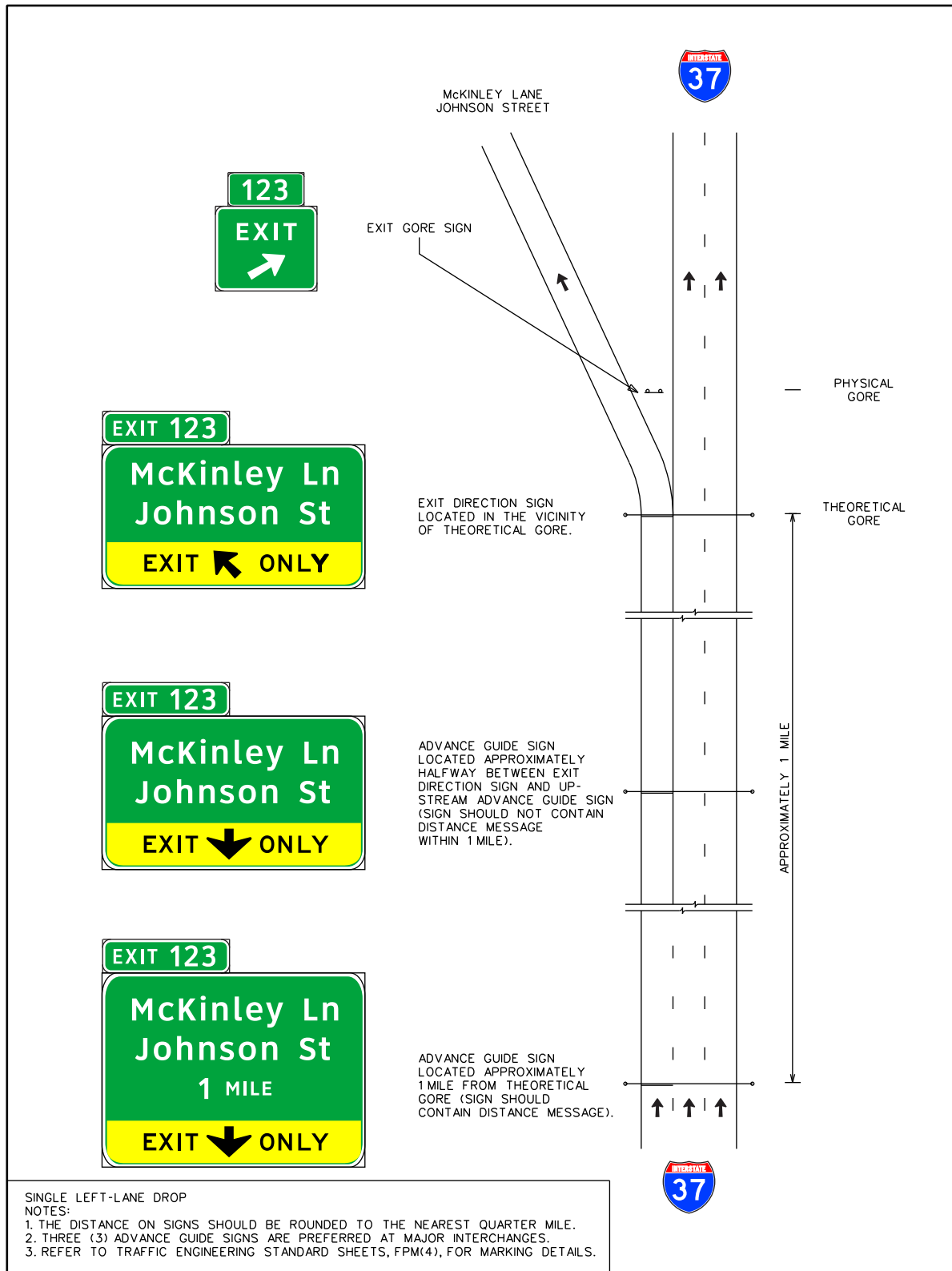
Figure 5-7. Signing for a single left-lane drop.
