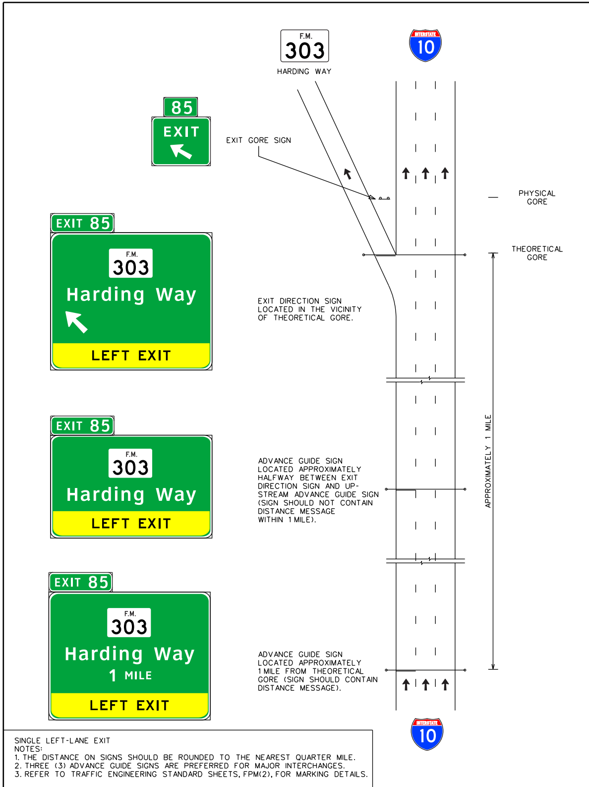
Figure 5-6. Signing for a single left-lane exit.
