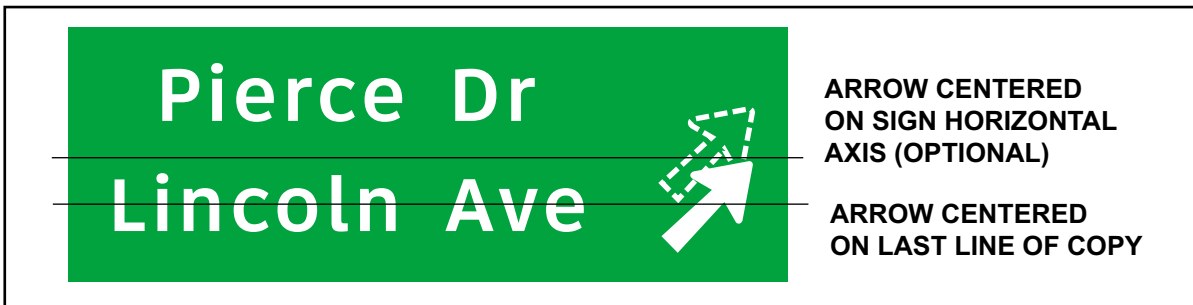
Figure 4-42. Arrow placement with two word messages, longest word message on the last line of copy, and arrow located to the right of the messages.
