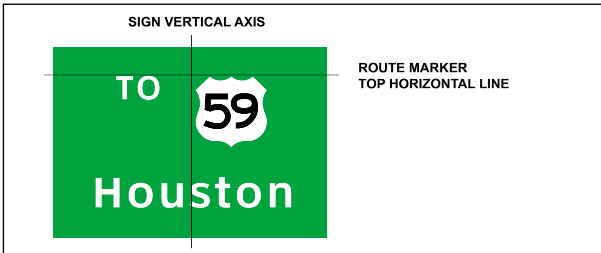
Figure 4-28. Route sign and TO placement.
