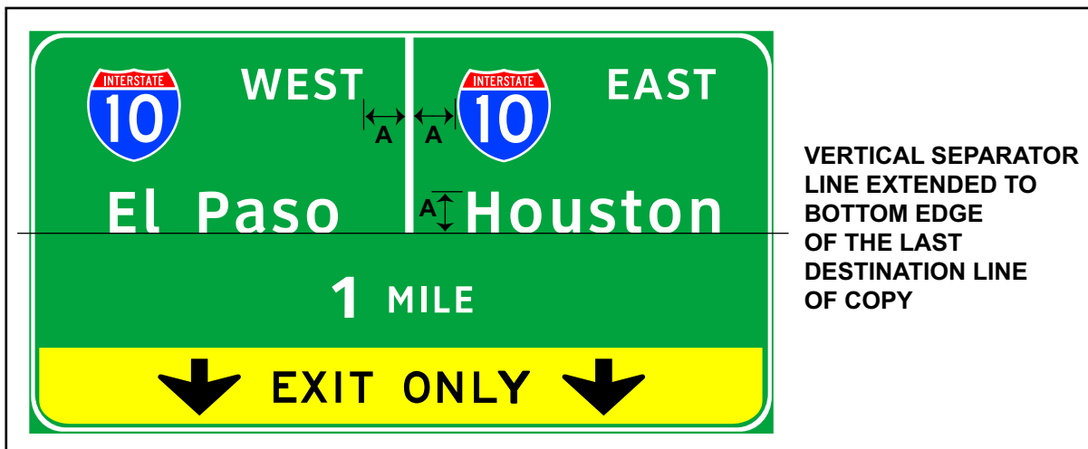
Figure 4-52. Spacing and placement of partial vertical separator line.
