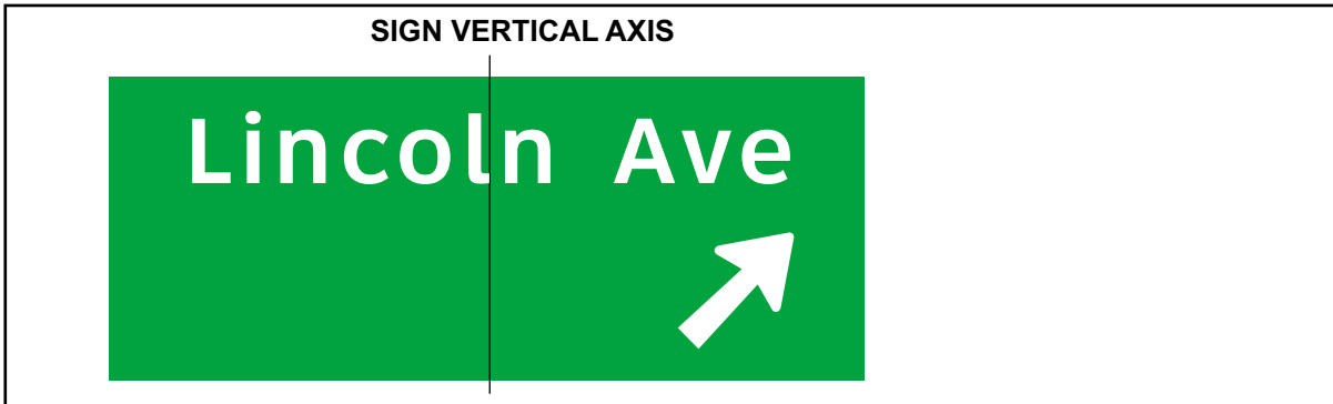
Figure 4-22. Word message placement on an Exit Direction sign.
