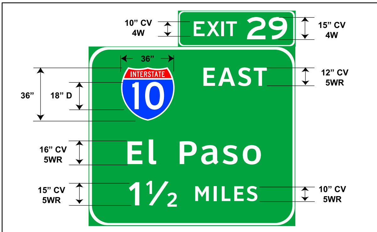
Figure 4-10. Letter style and minimum letter and numeral sizes on an Advance Guide sign.
