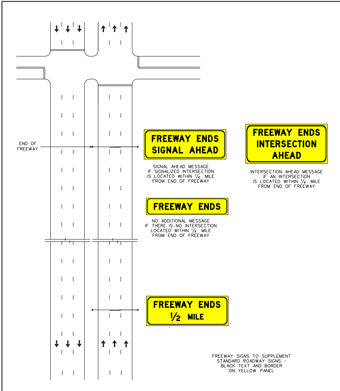
Figure 5-33. Freeway signing for a freeway-ends situation.
