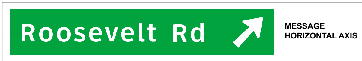
Figure 4-37. Arrow placement with word message on the same line of copy.
