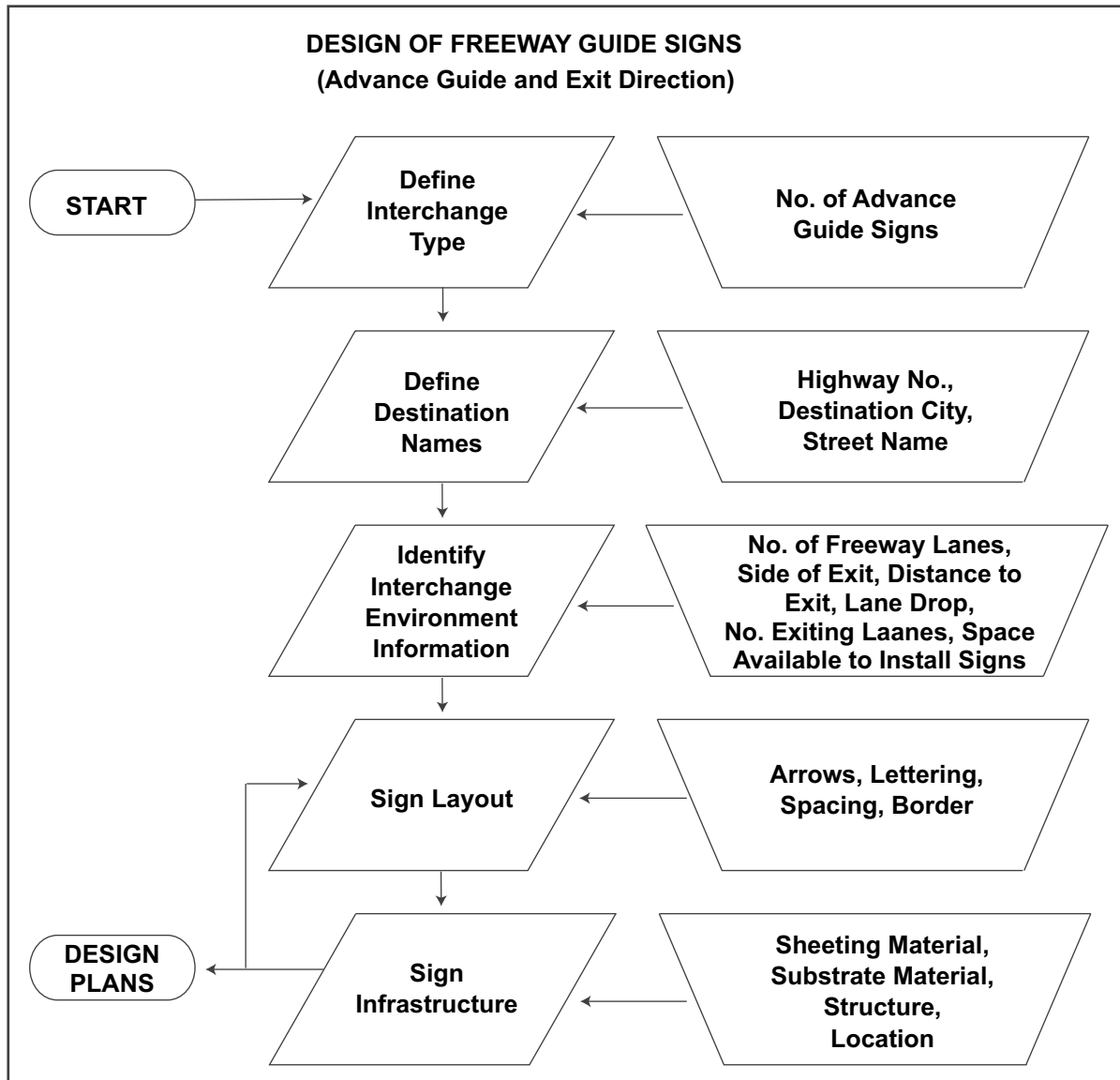
Figure 2-2. Advance Guide and Exit Direction sign design process.
