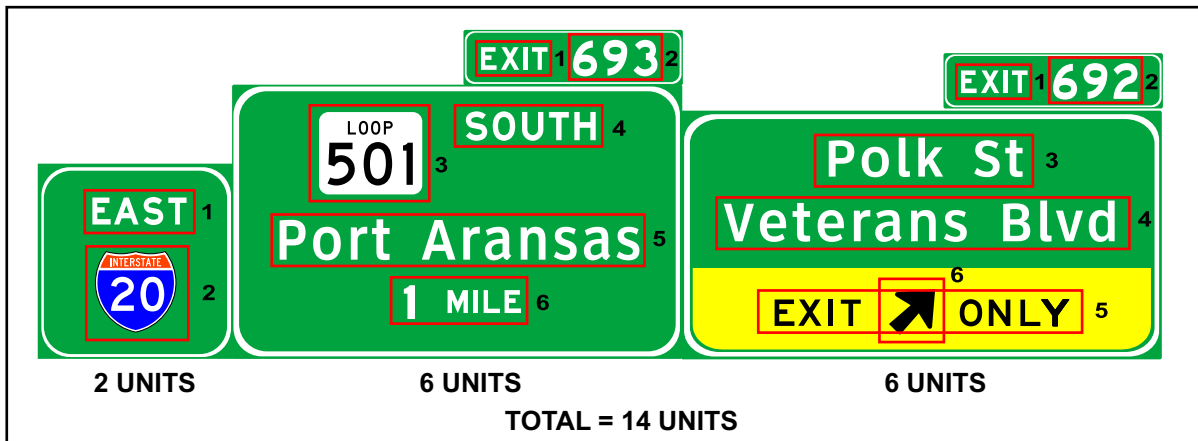
Figure 2-1. Example of sign information units.
