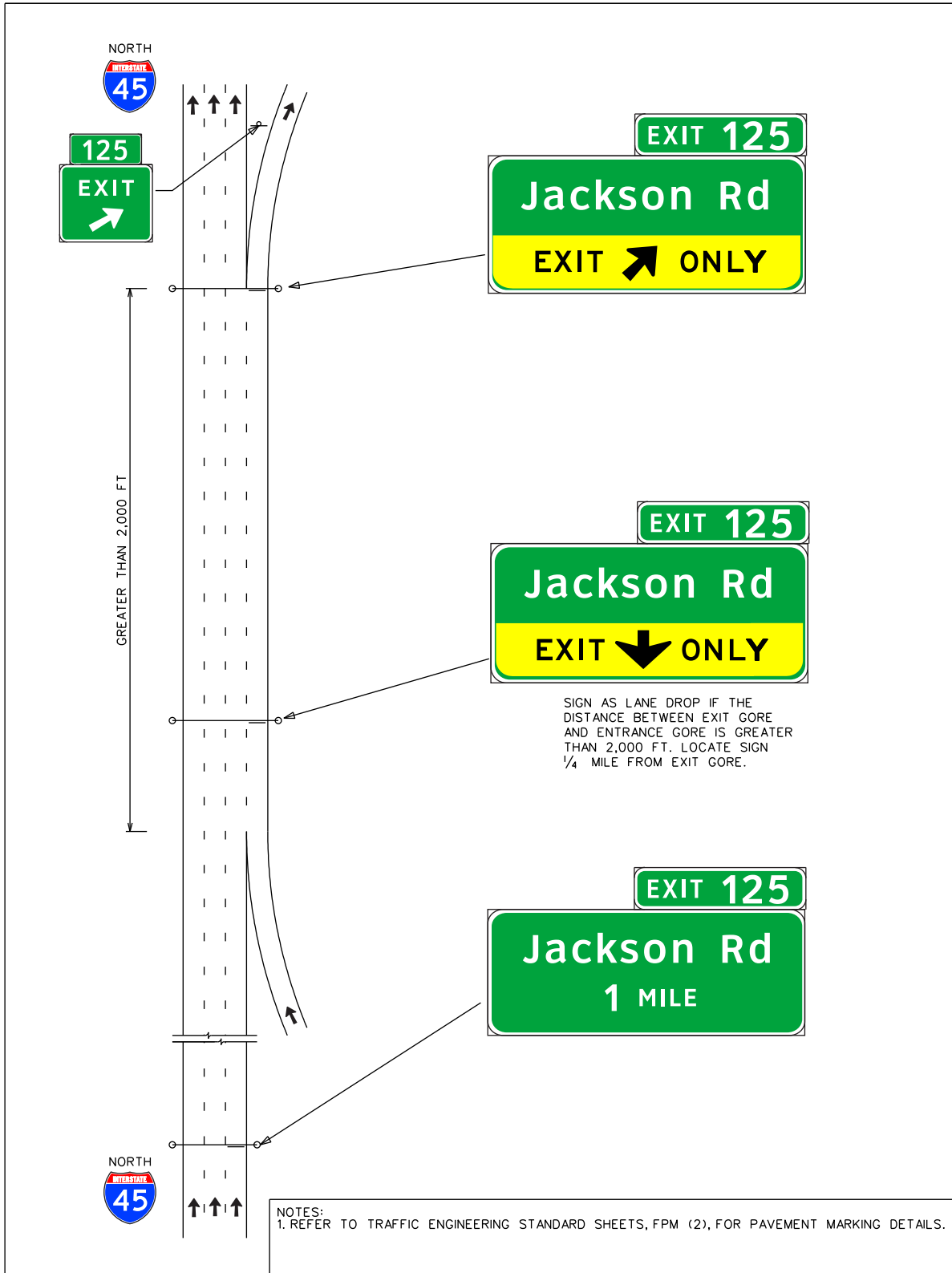
Figure 5-29. Closely spaced ramps with an added-lane entrance ramp and a lane drop exit ramp and greater than 2000 ft between exit and entrance ramp gores.
