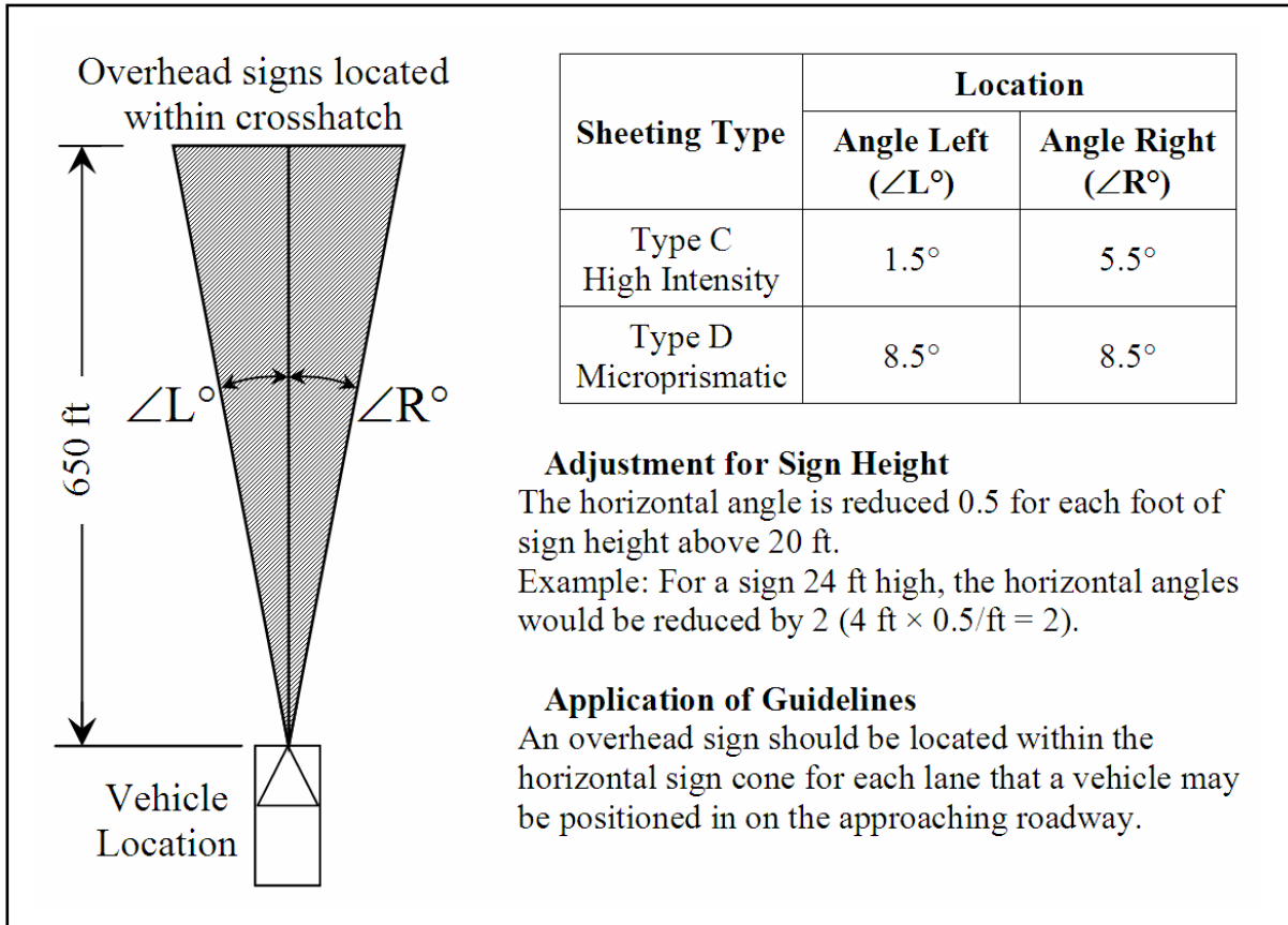
Figure A-1. Horizontal Sign Cone.
