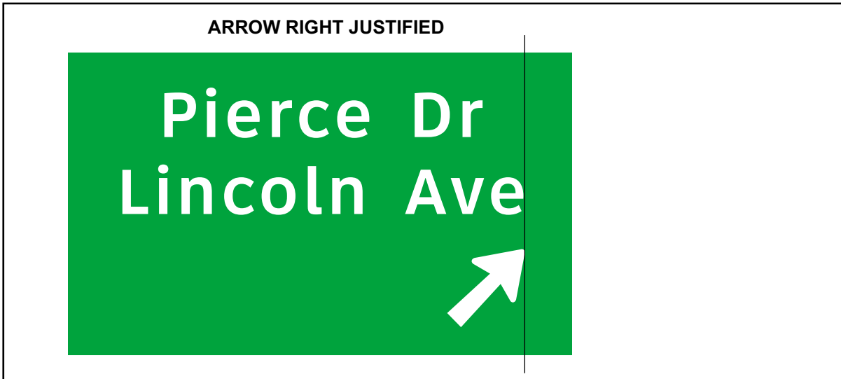
Figure 4-41. Preferred arrow placement with two word messages.
