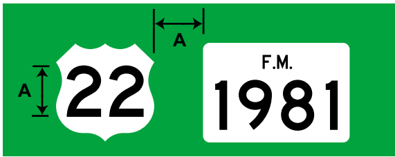
Figure 4-16. Lateral spacing between Route signs.
