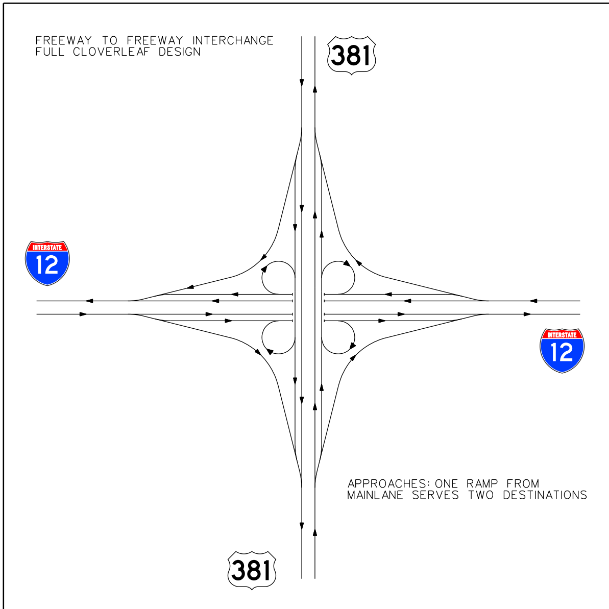
Figure 5-23. Cloverleaf interchange with collector-distributor roads.
