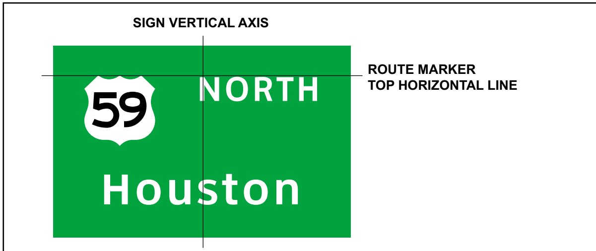
Figure 4-27. Route sign and cardinal direction placement.
