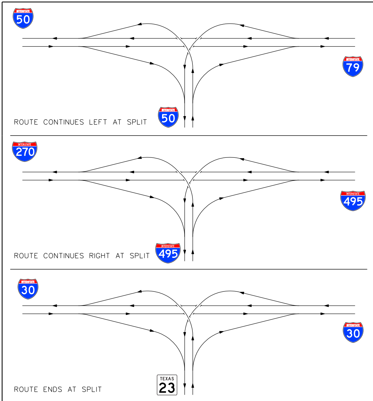
Figure 5-19. Three-leg directional interchanges with continuing and terminating routes.
