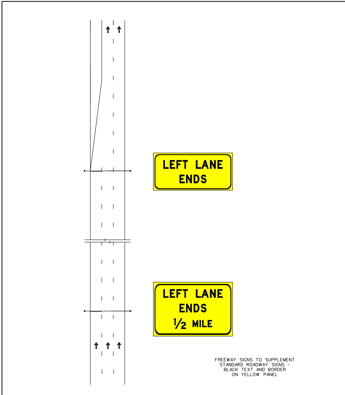
Figure 5-34. Freeway signing for a left-lane ends situation.
