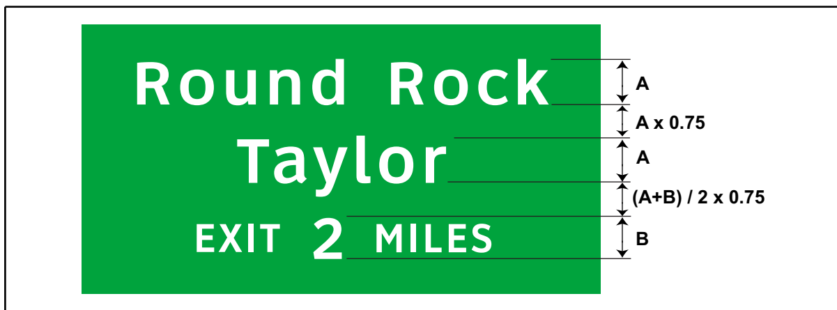
Figure 4-17. Interline spacing between word messages.
